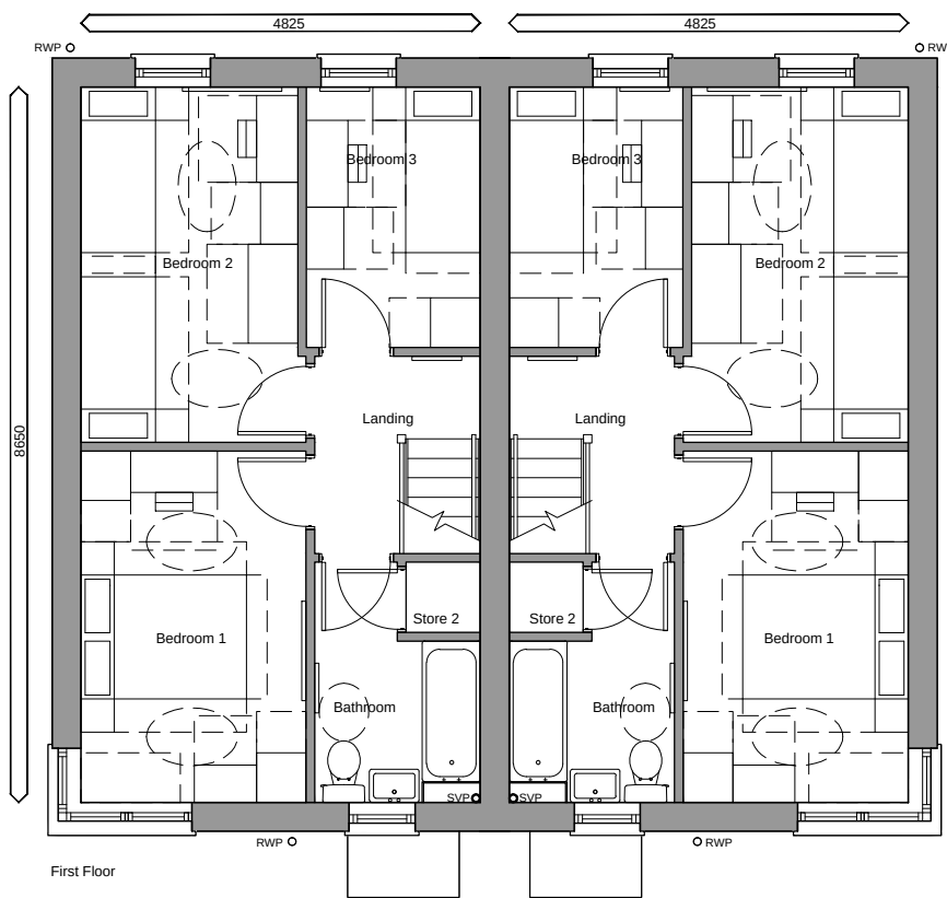
First Floor
