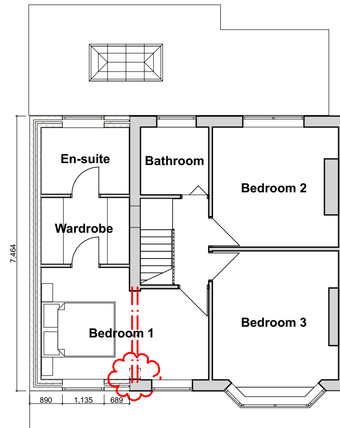
PROPOSED FIRST FLOOR 1:100
