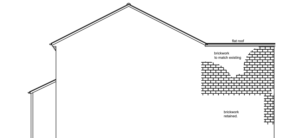
Proposed Opposite Side Elevation.
