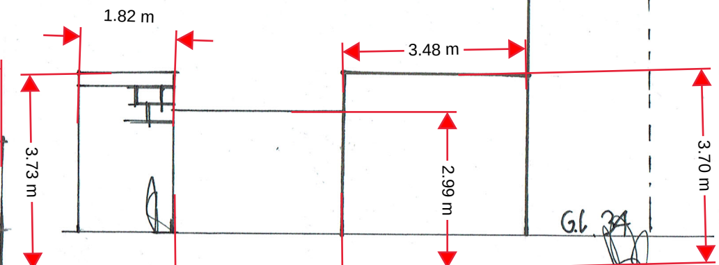
SIDE ELEVATION (FROM 32) PROPOSED
