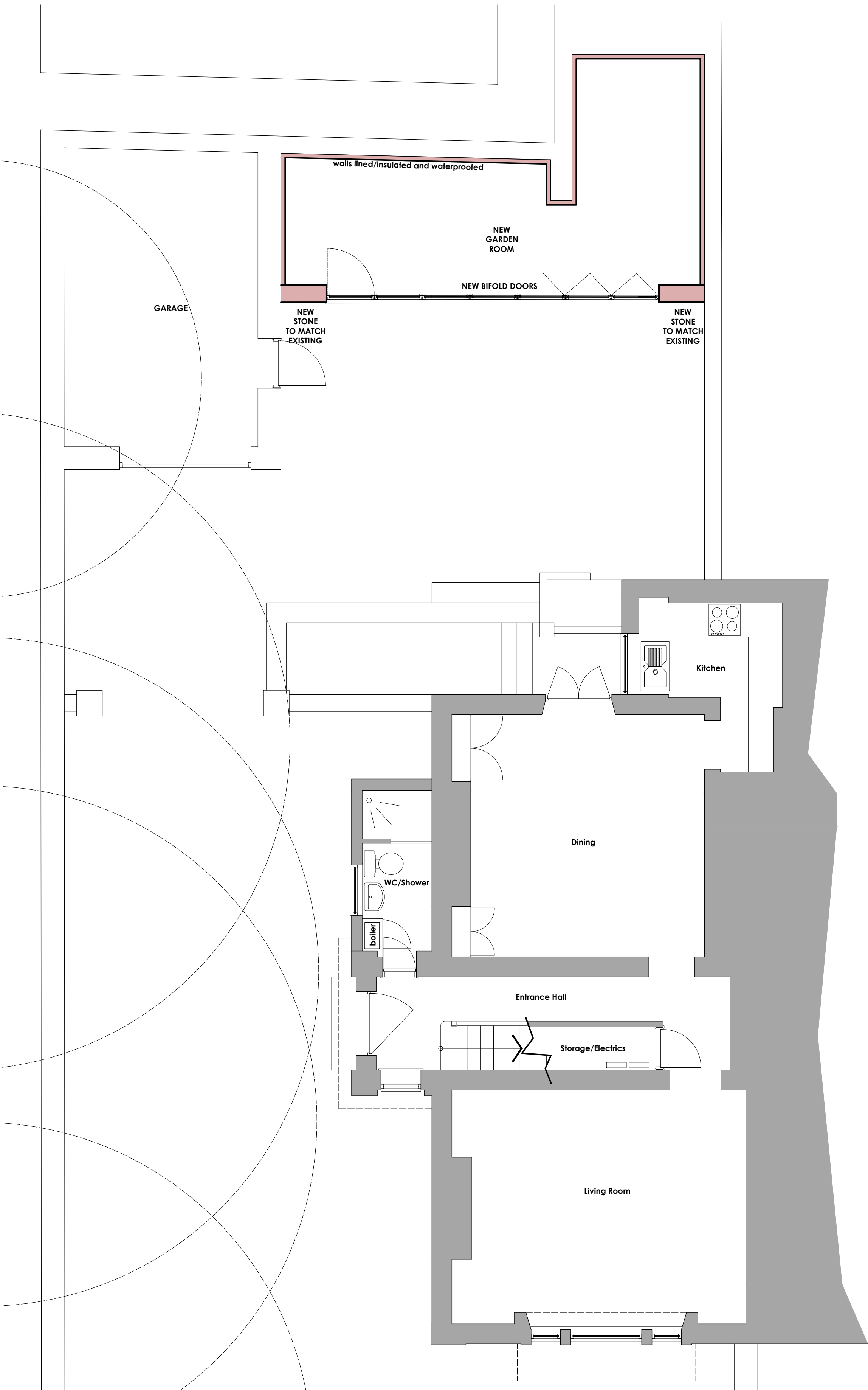
GROUND FLOOR - as proposed Scale 1:50 @ A1
