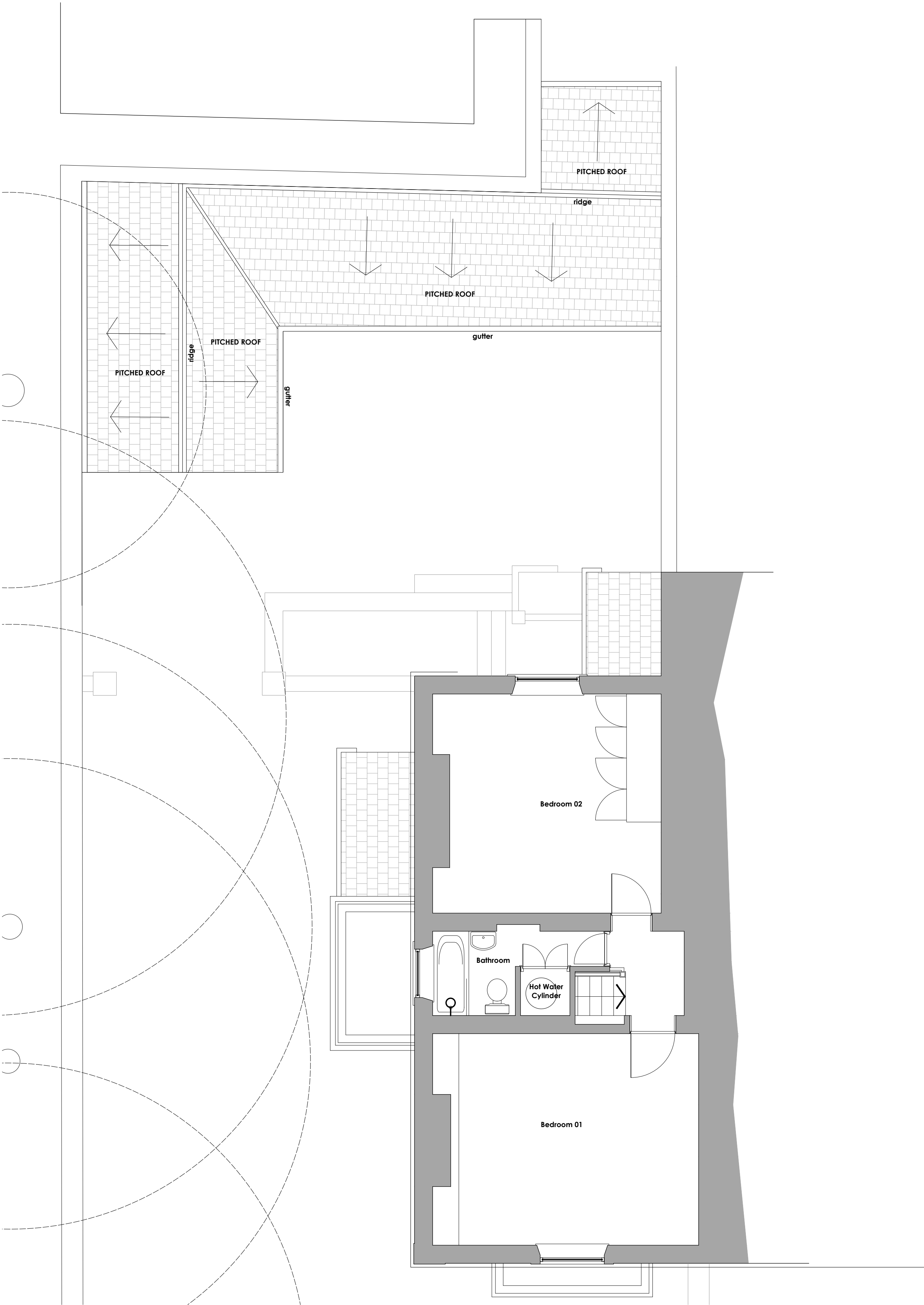
FIRST FLOOR - as proposed Scale 1:50 @ A1
