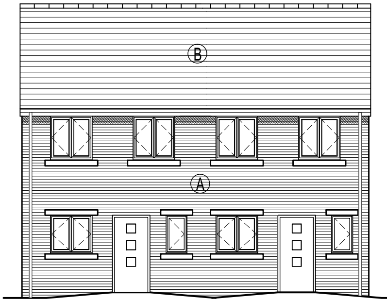
Plot 1+2 - Front
