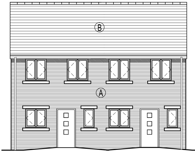
Plot 3+4 - Front
