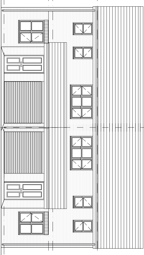
Front Elevation
