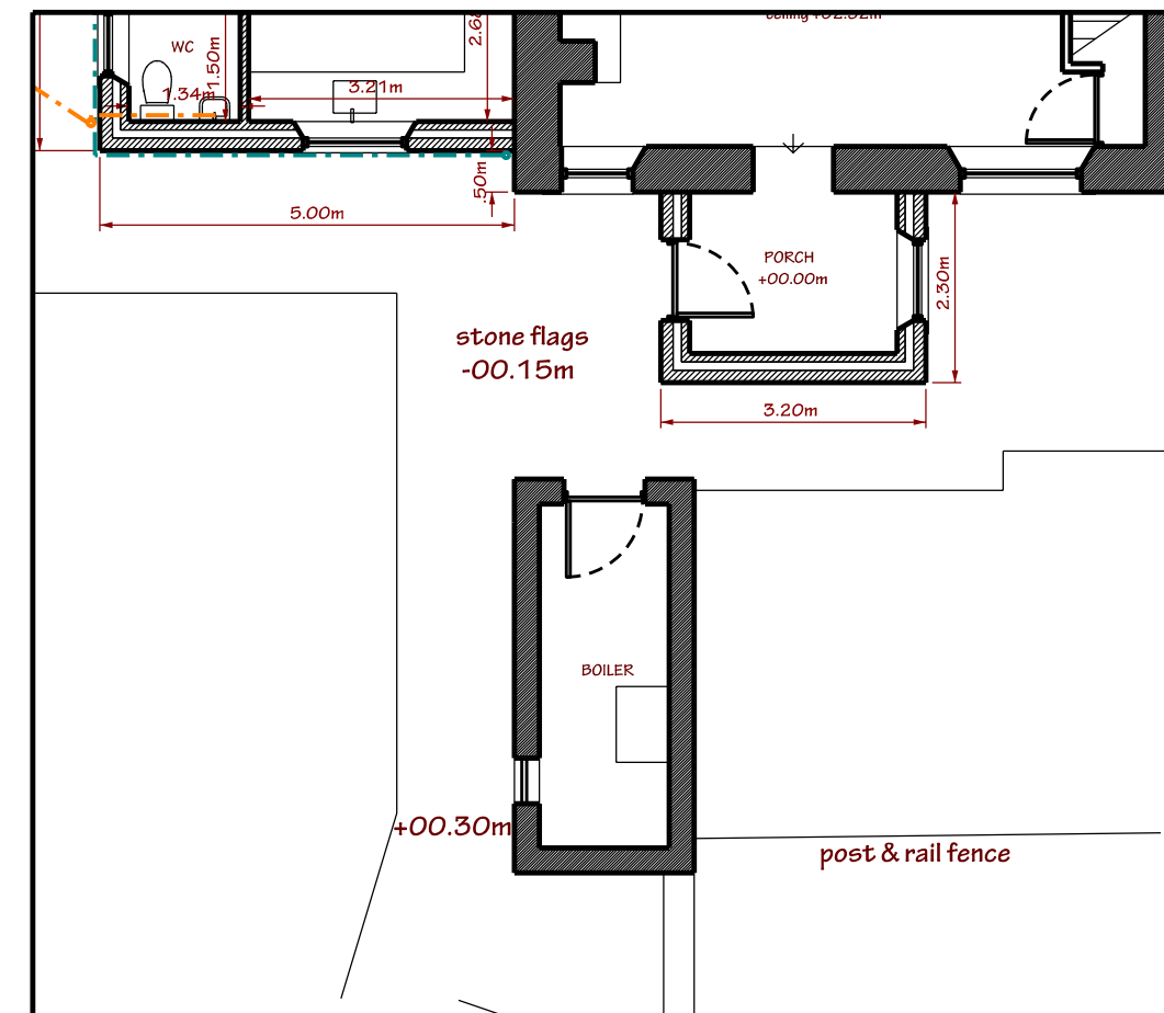
Plan Boiler Room - Proposed
