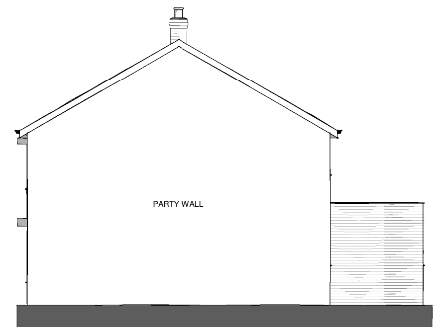
Right Side Elevation. 1 : 100
