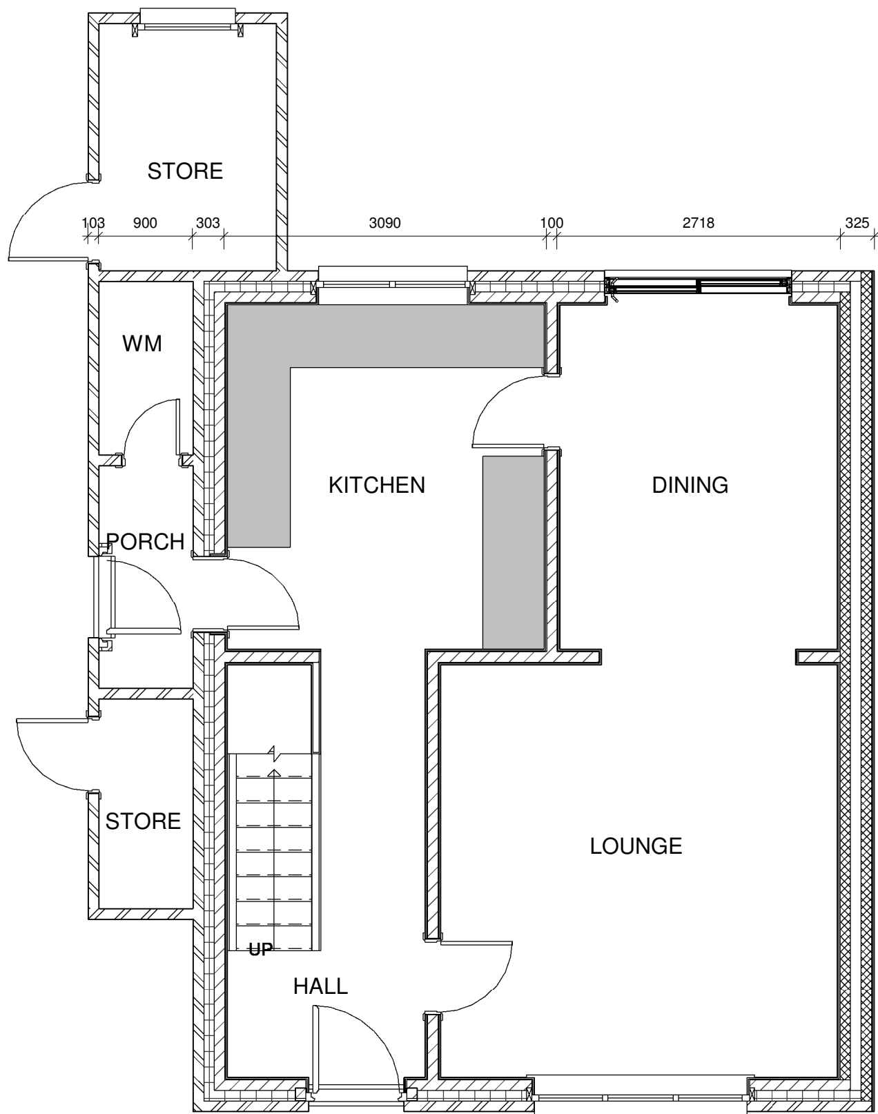
Existing Ground Floor G.A 1 : 50
