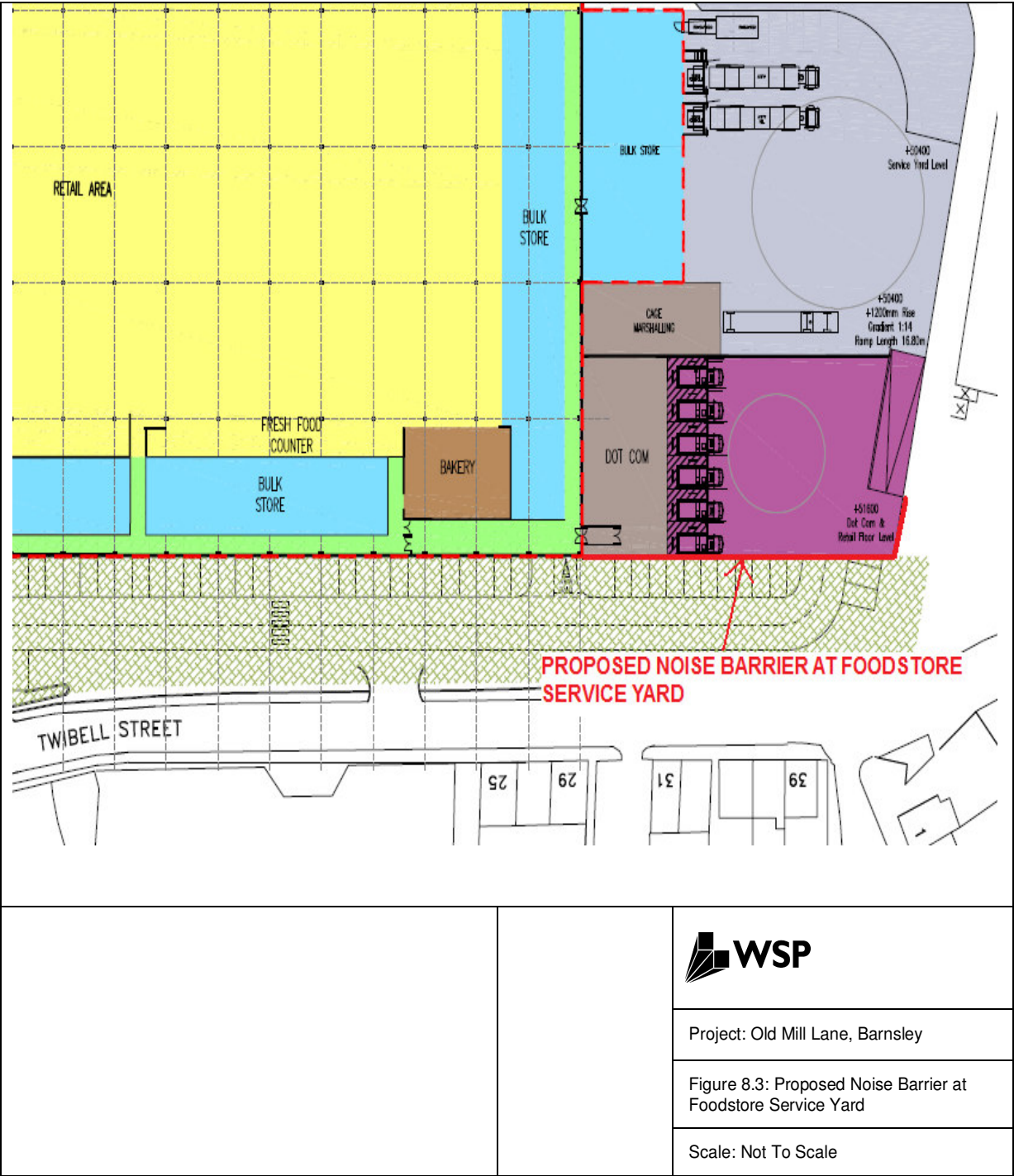
FIGURE 8.3: PROPOSED NOISE BARRIER AT FOODSTORE SERVICE YARD
