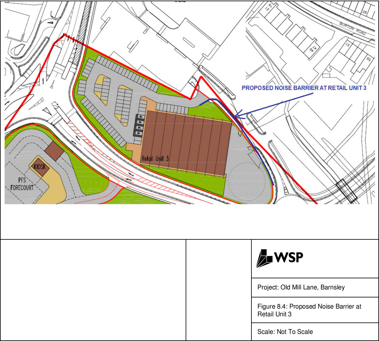
FIGURE 8.4: PROPOSED NOISE BARRIER AT RETAIL UNIT 3
