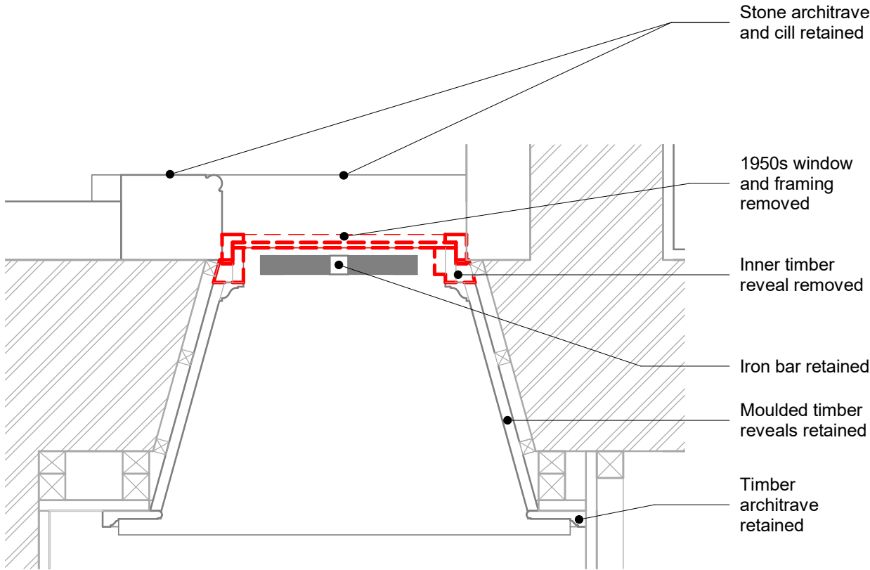
3 JC20 - Window Opening Removal
