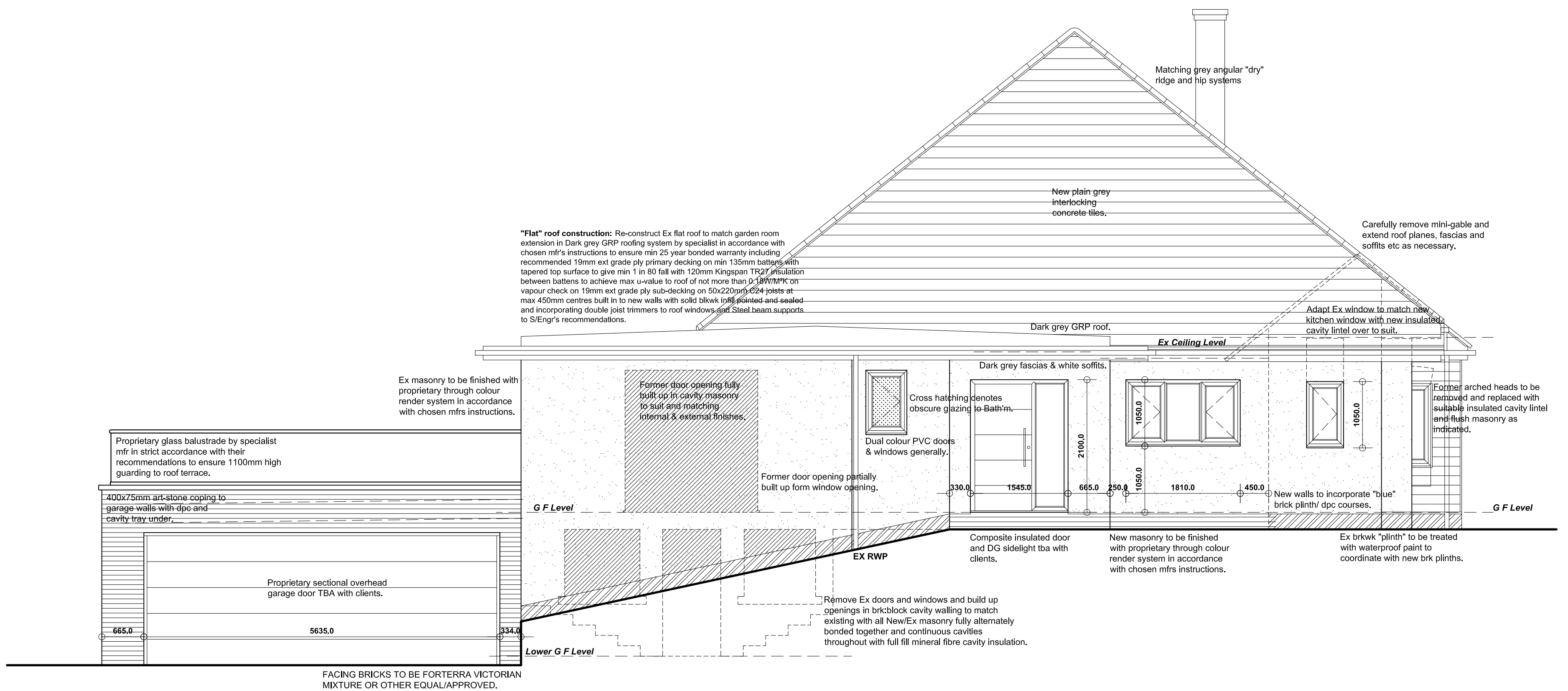
SIDE (NW) ELEVATION
