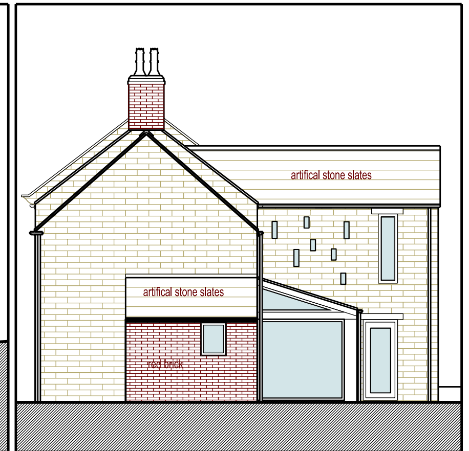
East Elevation - Proposed
