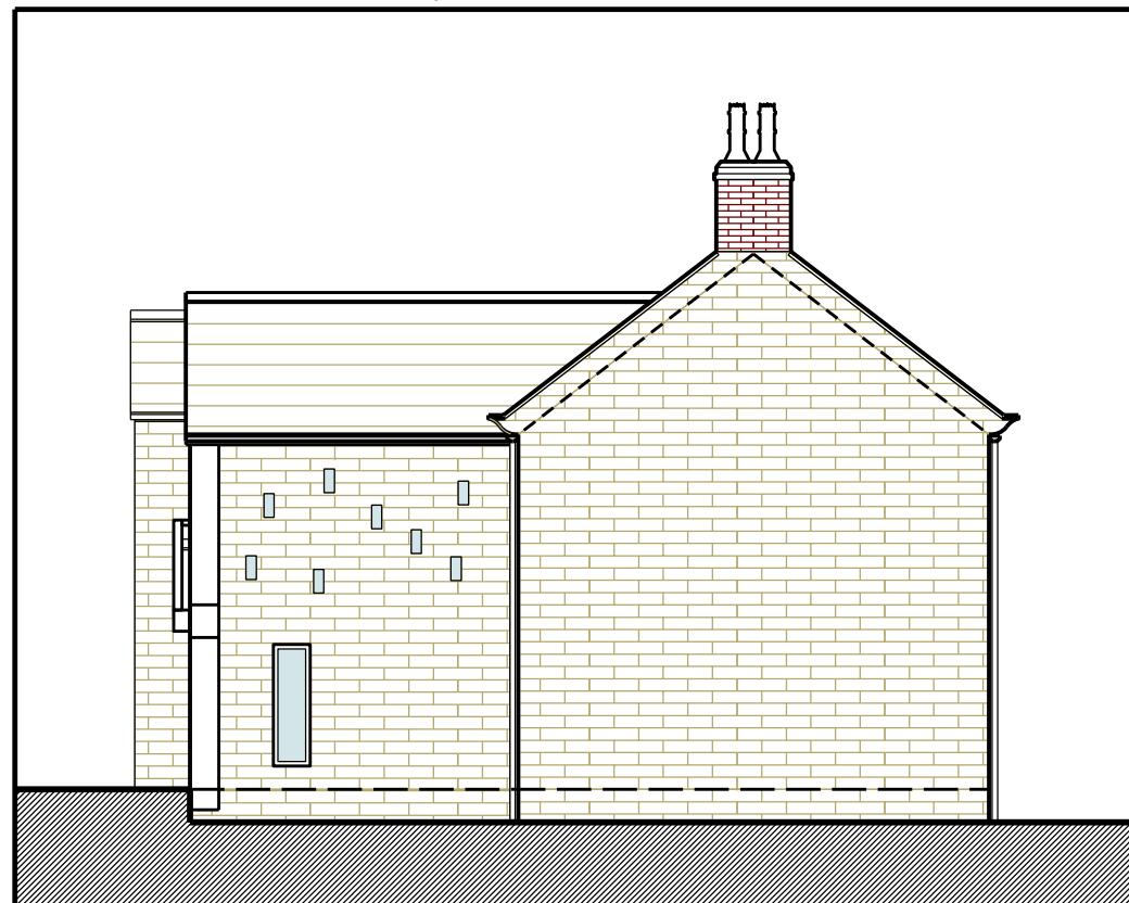
West Elevation - Proposed
