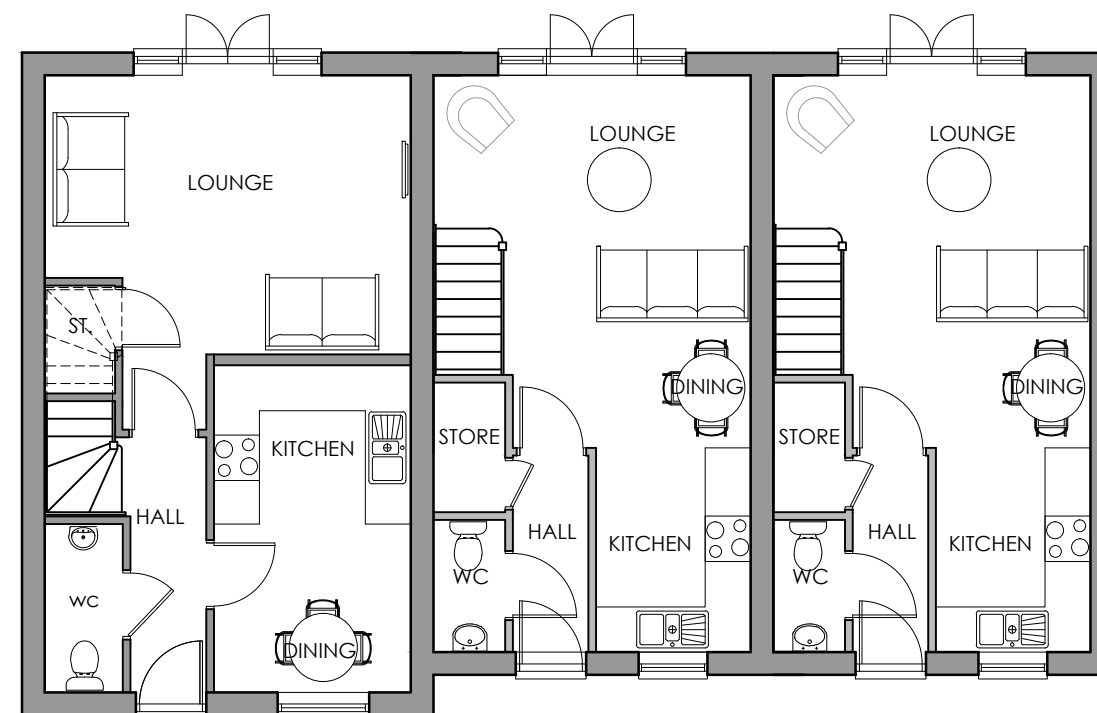
Type 83 GROUND FLOOR PLAN
