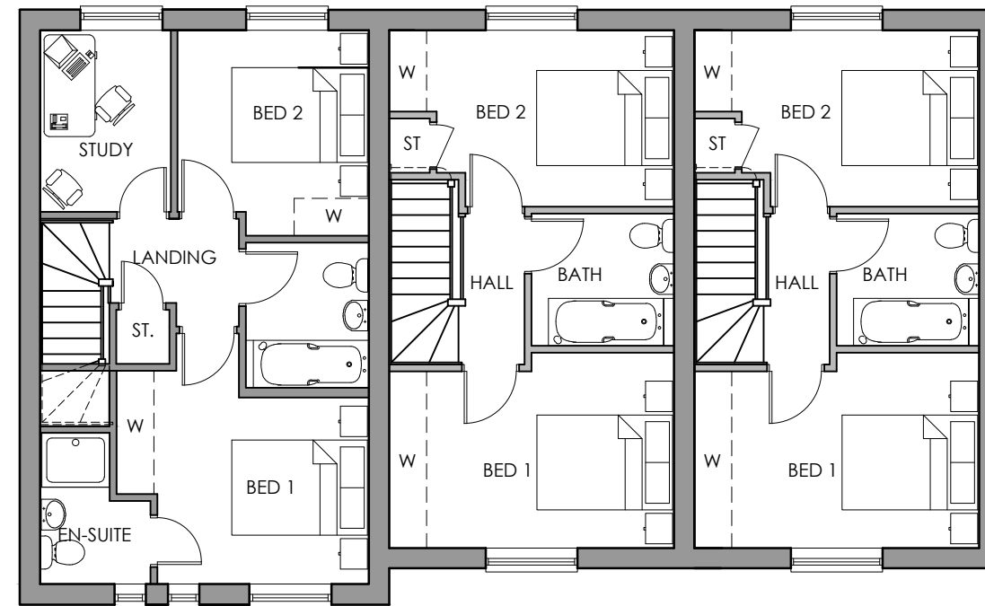
Type 83 FIRST FLOOR PLAN
