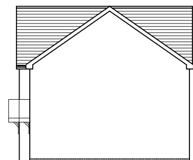
Type 68 SIDE ELEVATION
