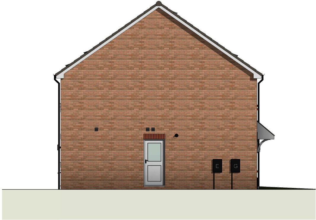
2 Gable Elevation 1 : 100
