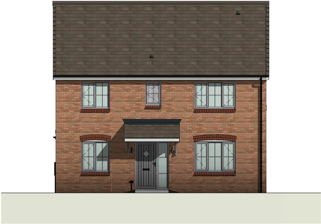
1 Front Elevation 1 : 100
