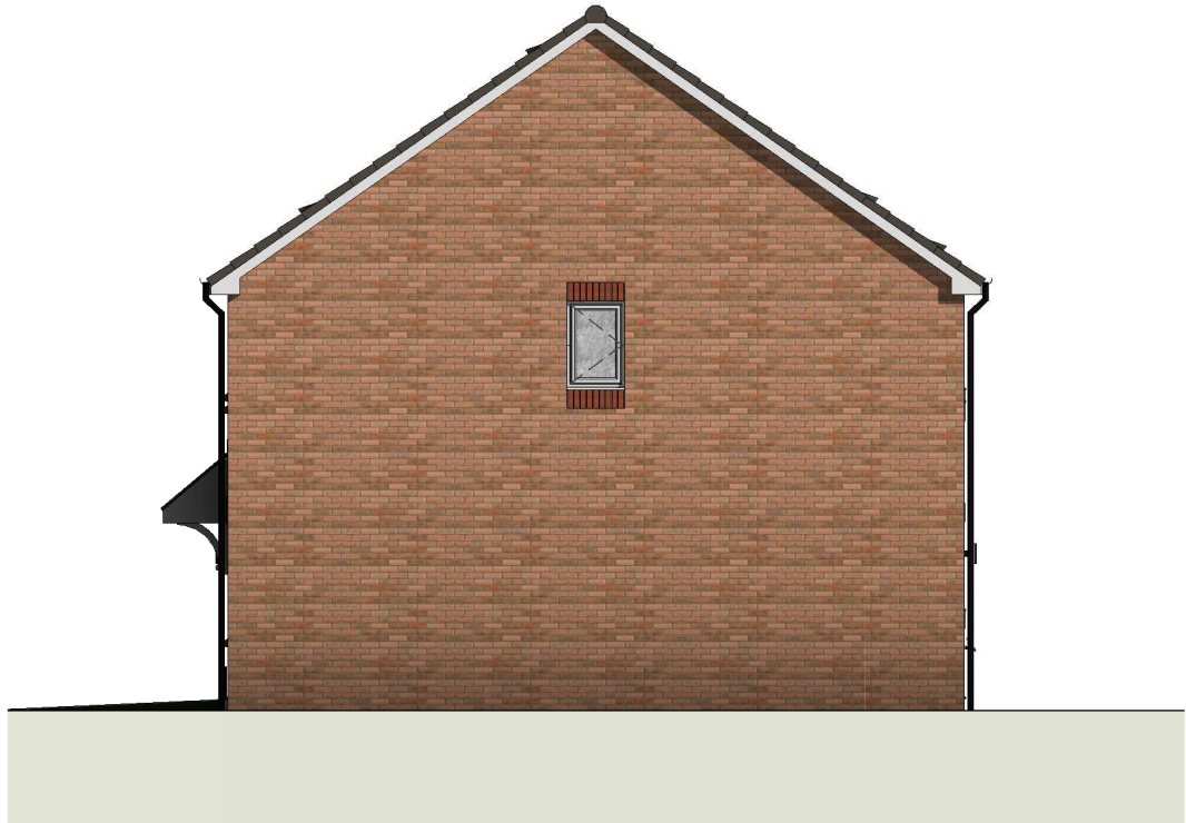
4 Gable Elevation 1 : 100
