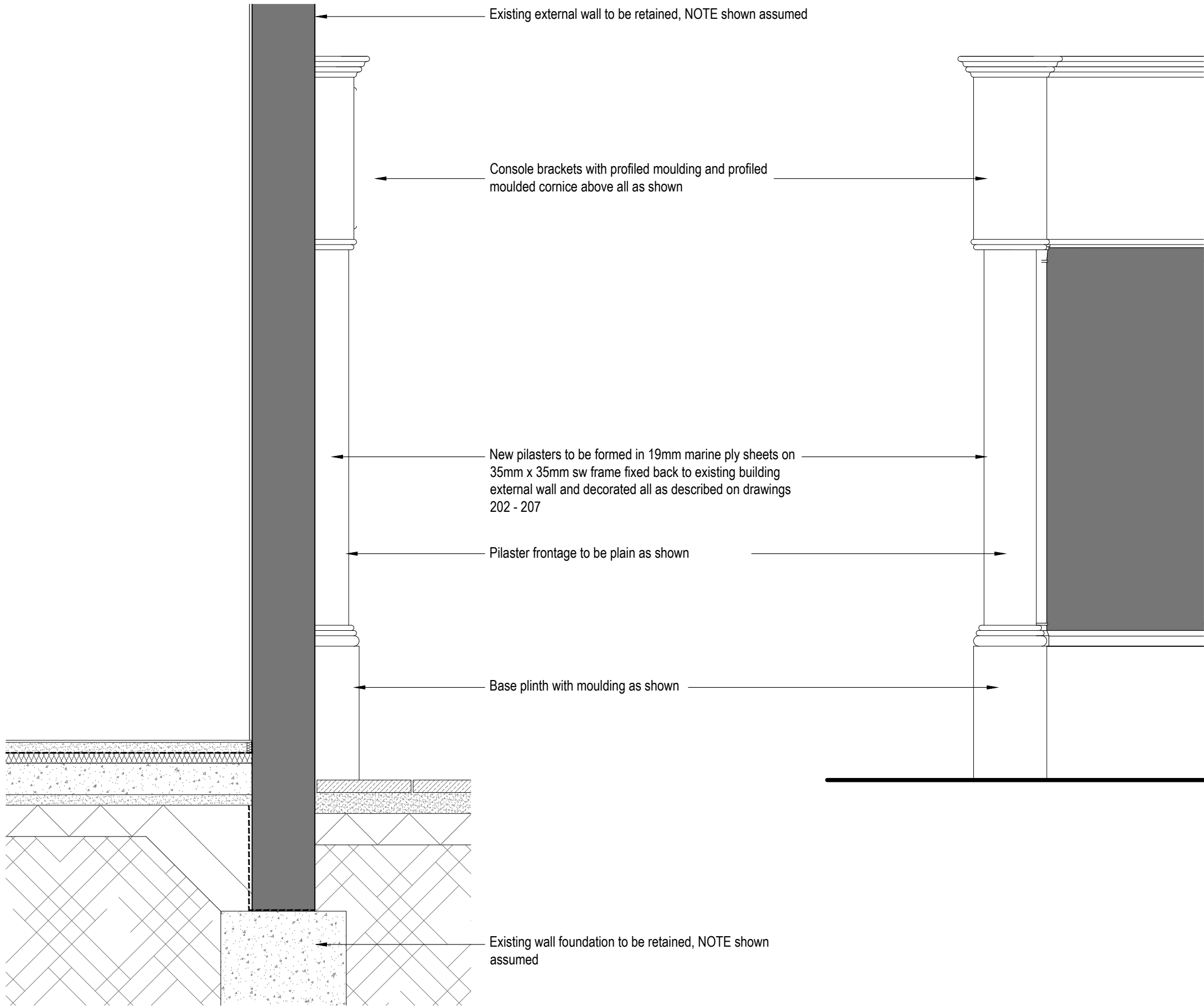
Typical Pilaster Side Elevation
