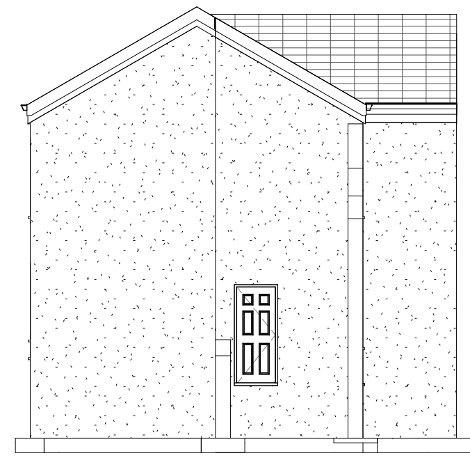
2 Existing Rear Elevation 1 : 100
