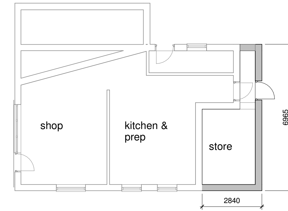
12 Proposed Ground Floor 1 : 100
