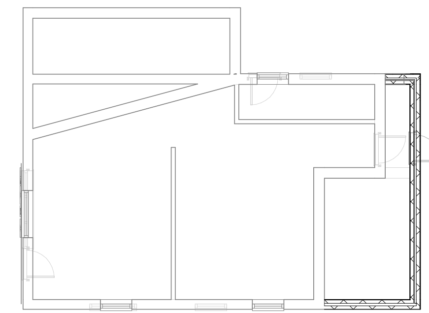
13 Proposed First Floor 1 : 100
