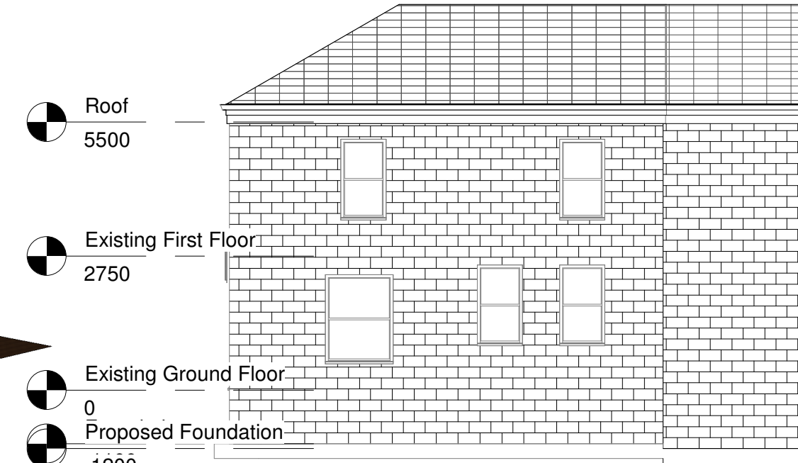
10 Proposed South 1 : 100
