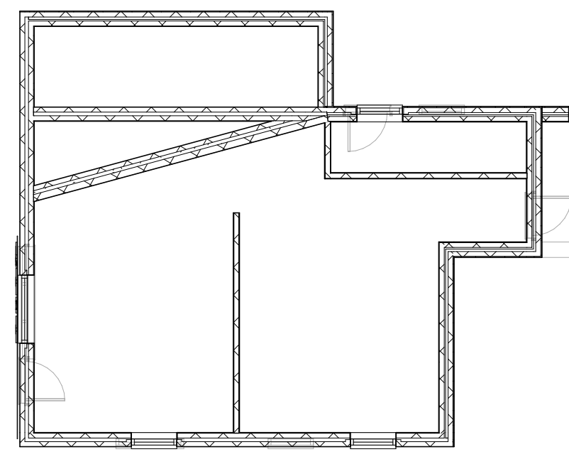
6 Existing First Floor 1 : 100
