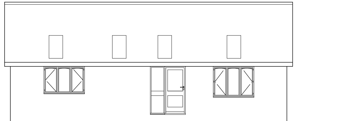
FRONT ELEVATION
