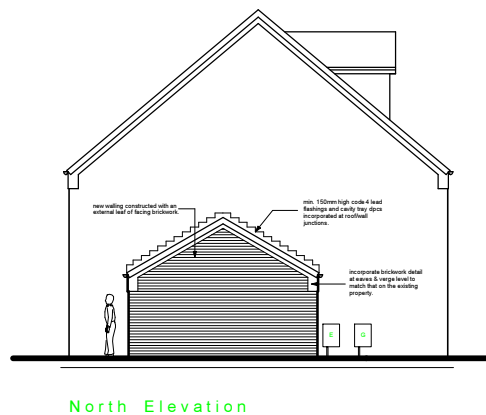
North Elevation
