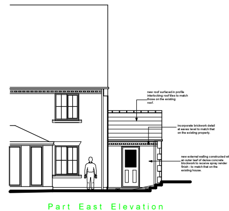
Part East Elevation
