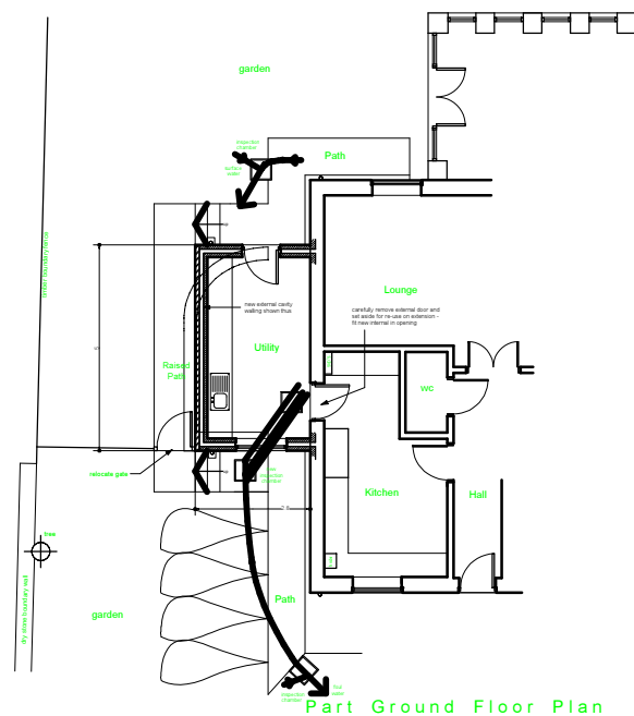
Part Ground Floor Plan
