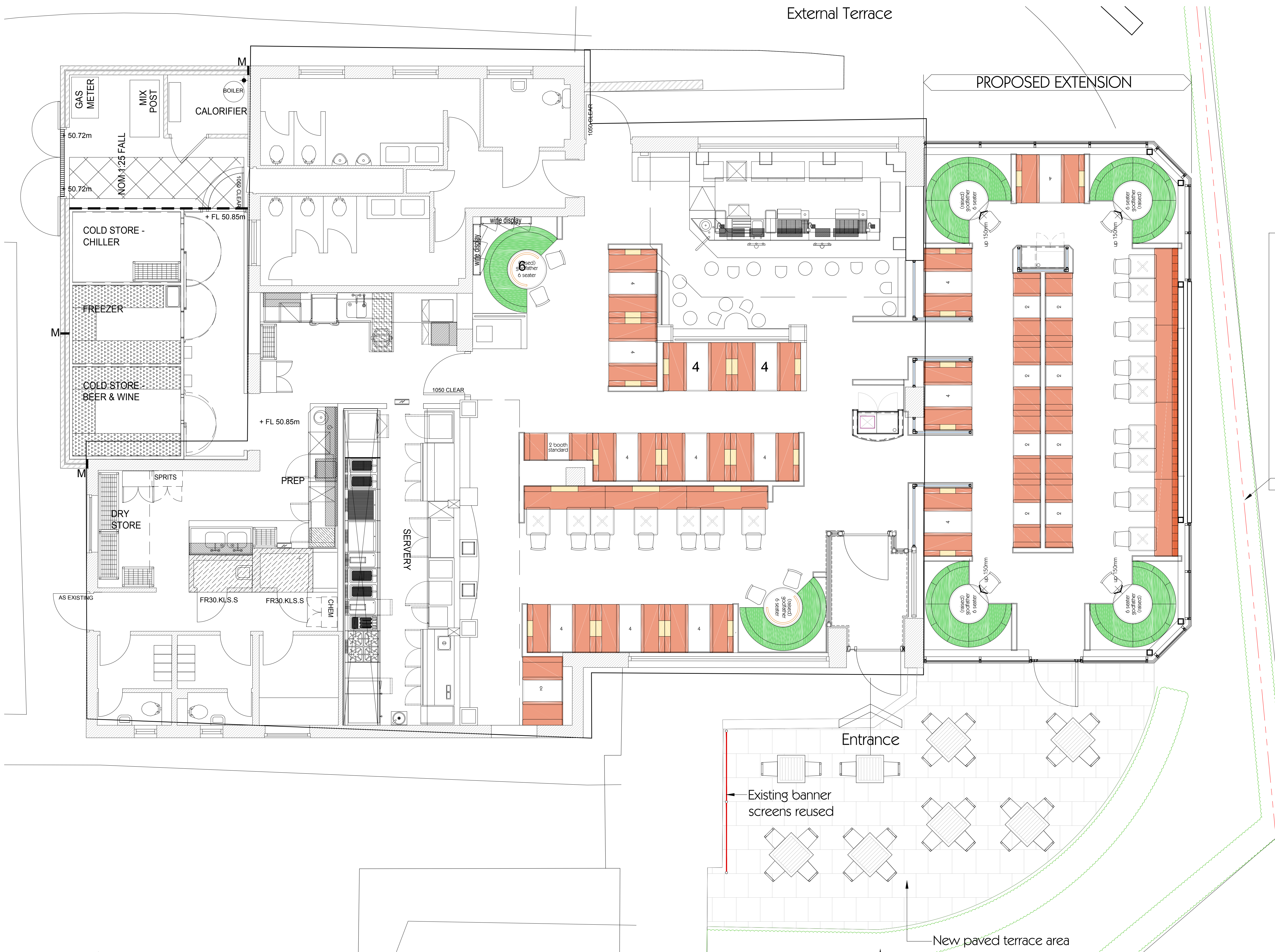
Layout Plan scale 1/100 @ A1, 1/200 @ A3
