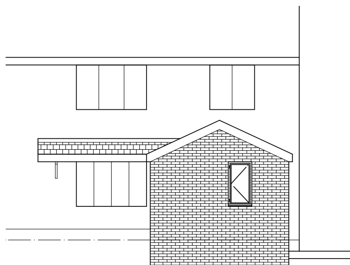
FRONT ELEVATION
