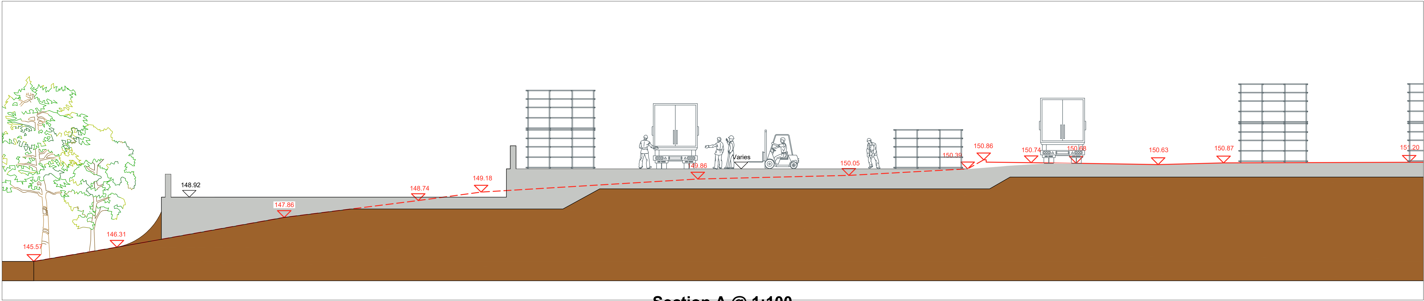
Section A @ 1:100
