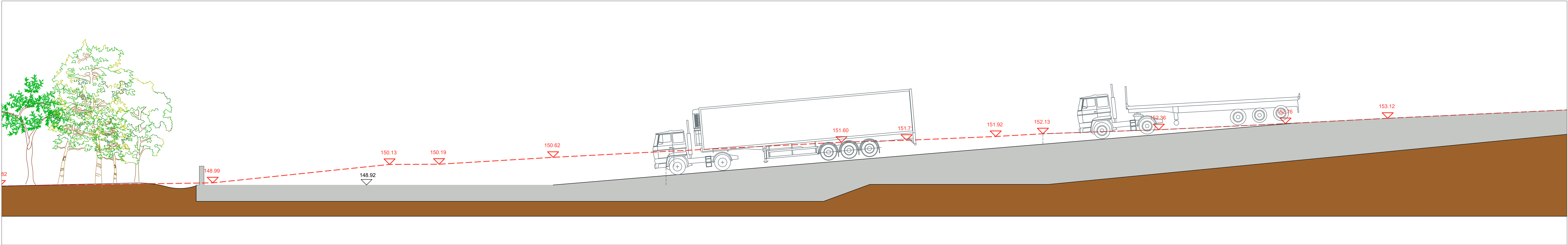
Section C Along Gradient Ramp 1:12 @ 1:100
