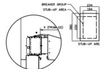
BREAKER STUB-UP LOCATION
