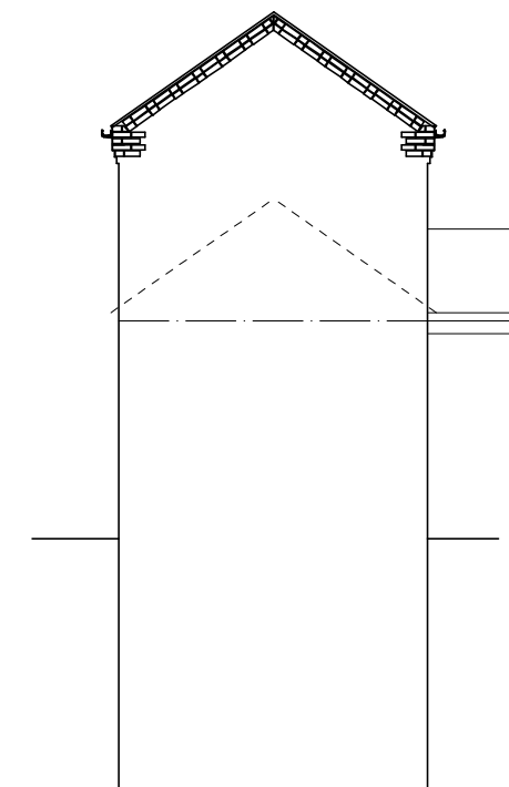
Front Elevation - 1:100
