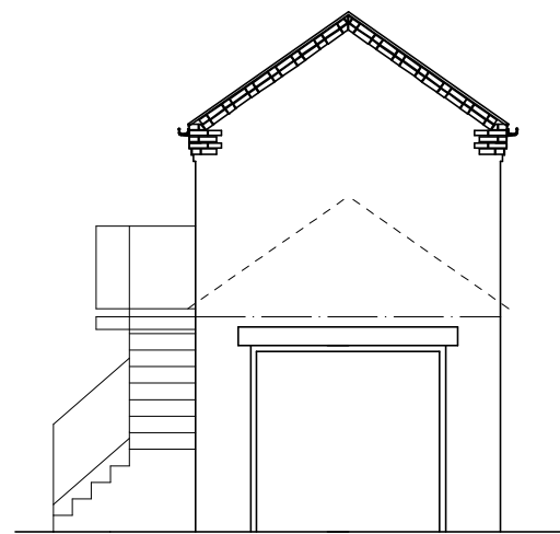
Front Elevation - 1:100
