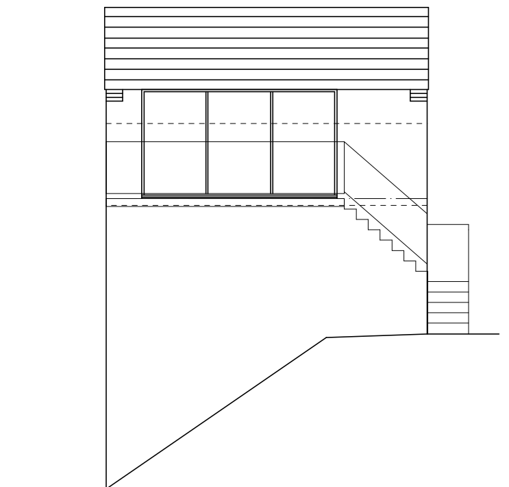
Side Elevation - 1:100
