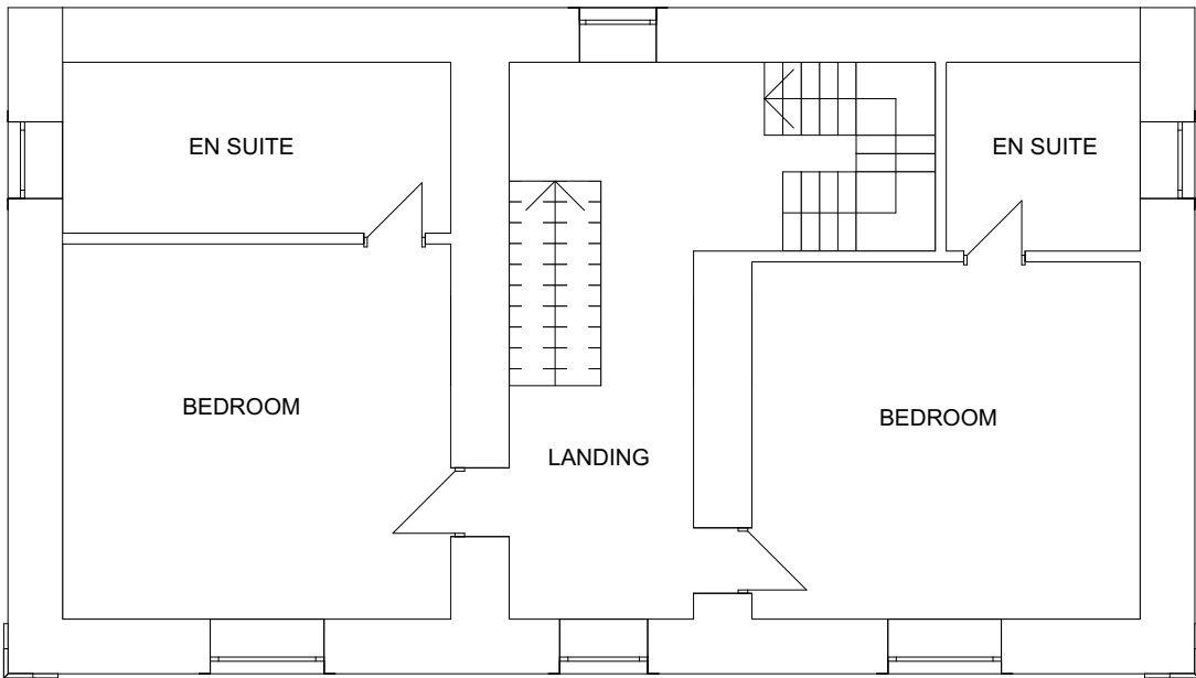
1. First Floor Proposed 1:100
