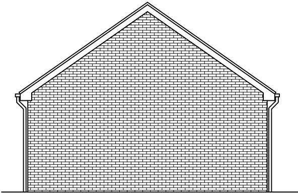
PROPOSED SIDE ELEVATION SCALE 1:100 AT A3
