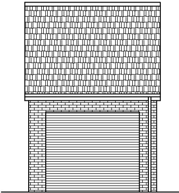
PROPOSED FRONT ELEVATION SCALE 1:100 AT A3
