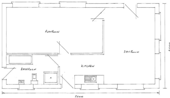
PROPOSED PLAN SCALE 1:50
