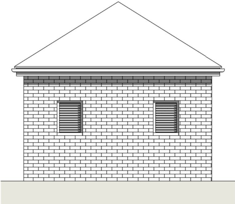
External Scooter Store - GA Rear Elevation 1 : 50
