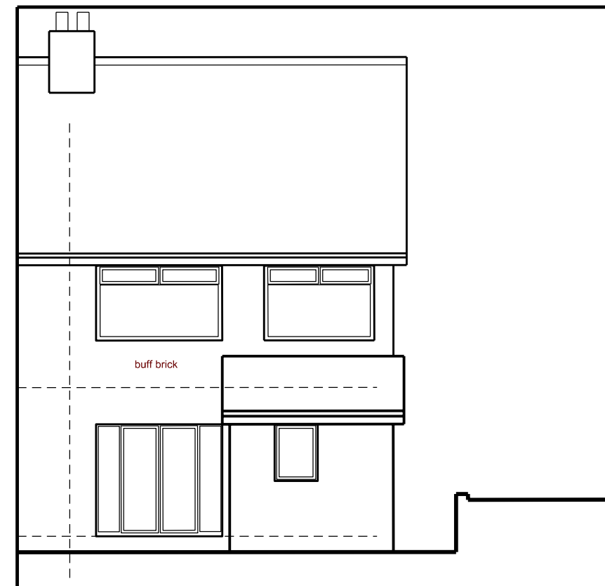
South Elevation - Existing
