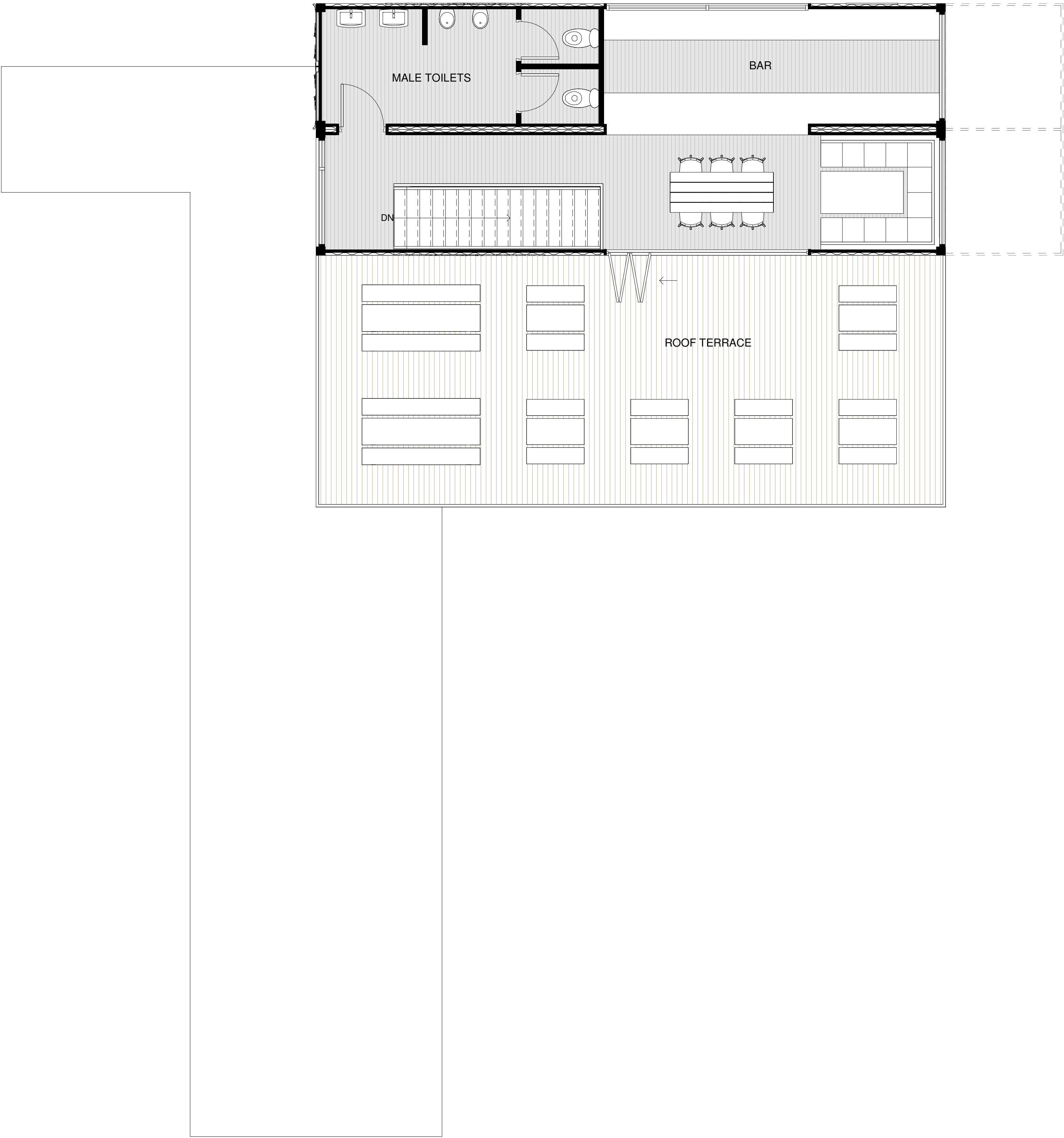
PROPOSED FIRST FLOOR 1 : 50
