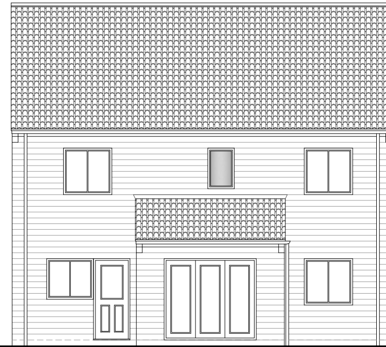
REAR ELEVATION
