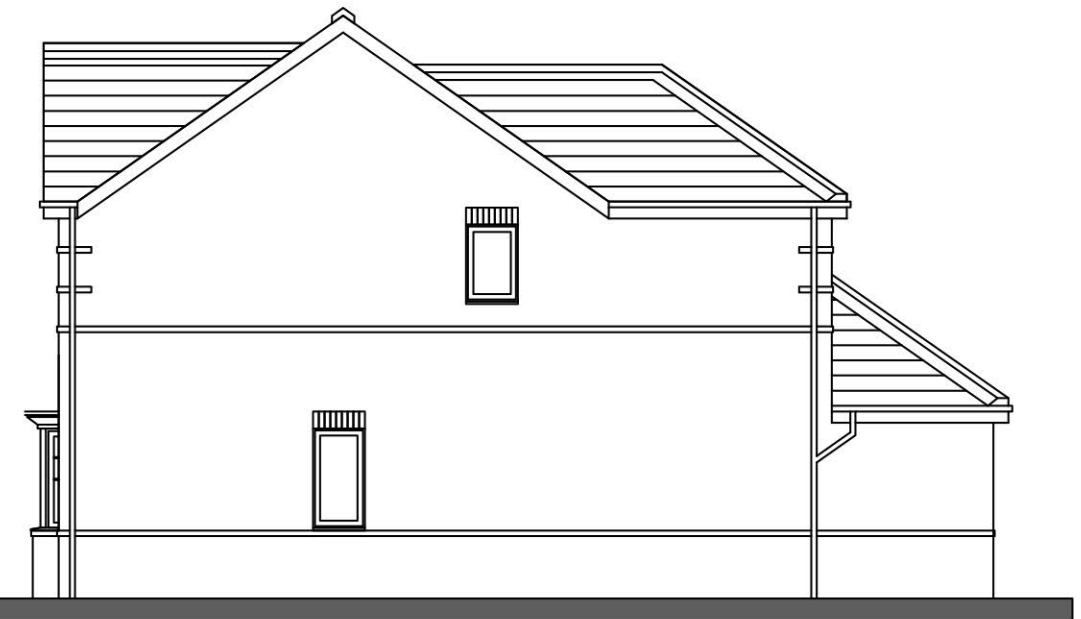
SIDE ELEVATION
