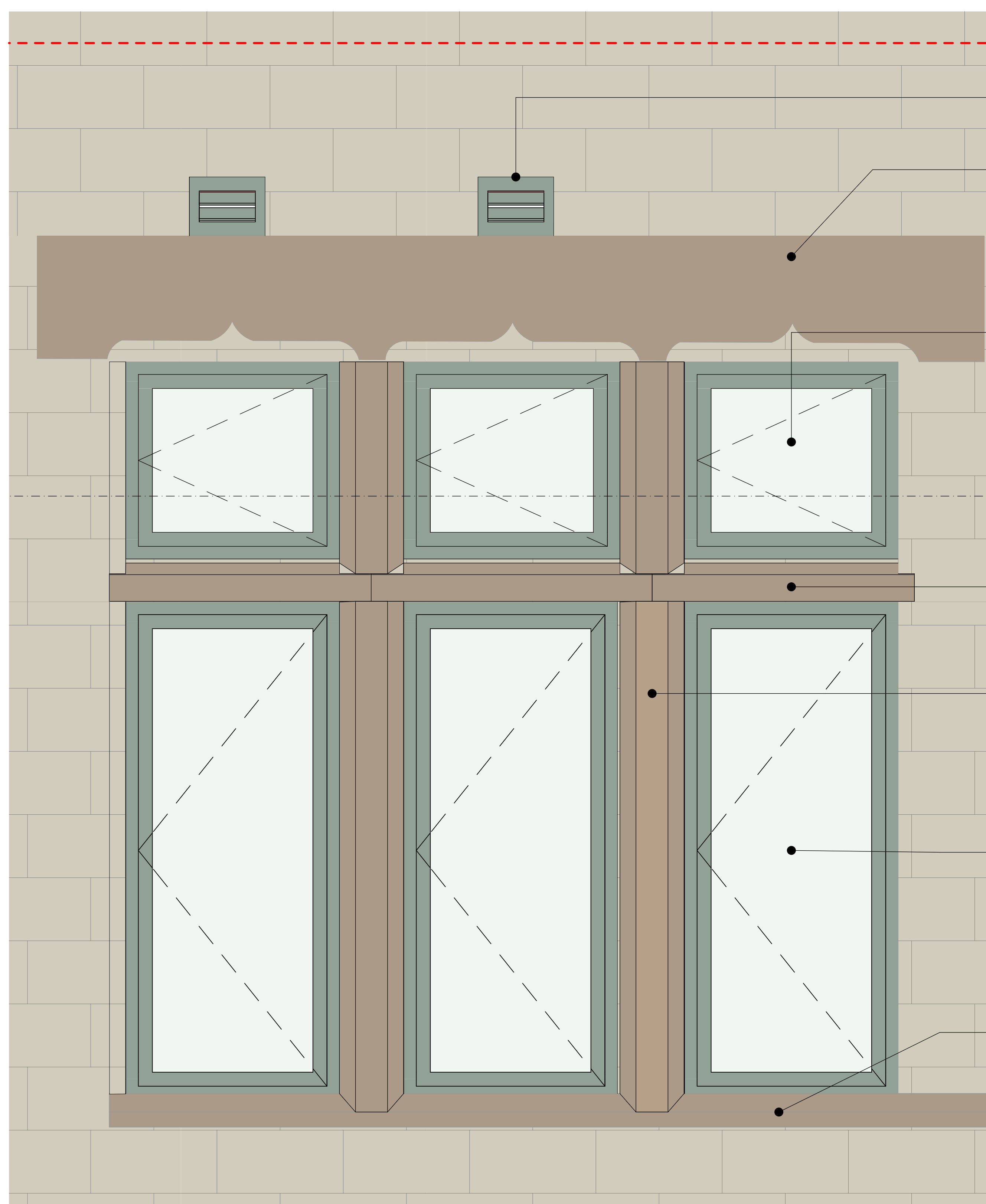
Typical New Window Installed Into Existing Opening: Side-Hung, Outward Opening Casement Window, Triple Glazed 1:10
