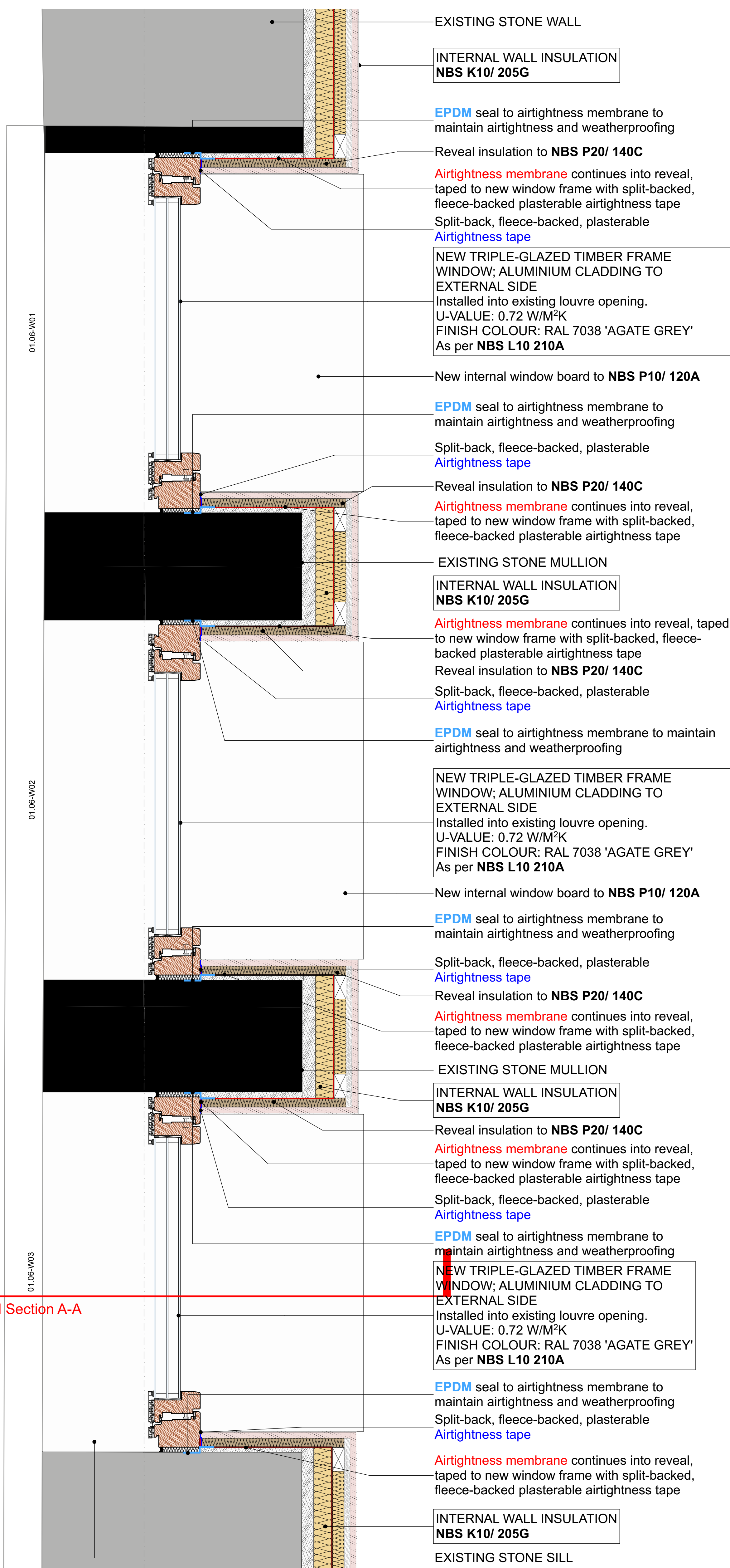
Typical New Side-Hung Outward Opening Window Plan Detail 1:5
