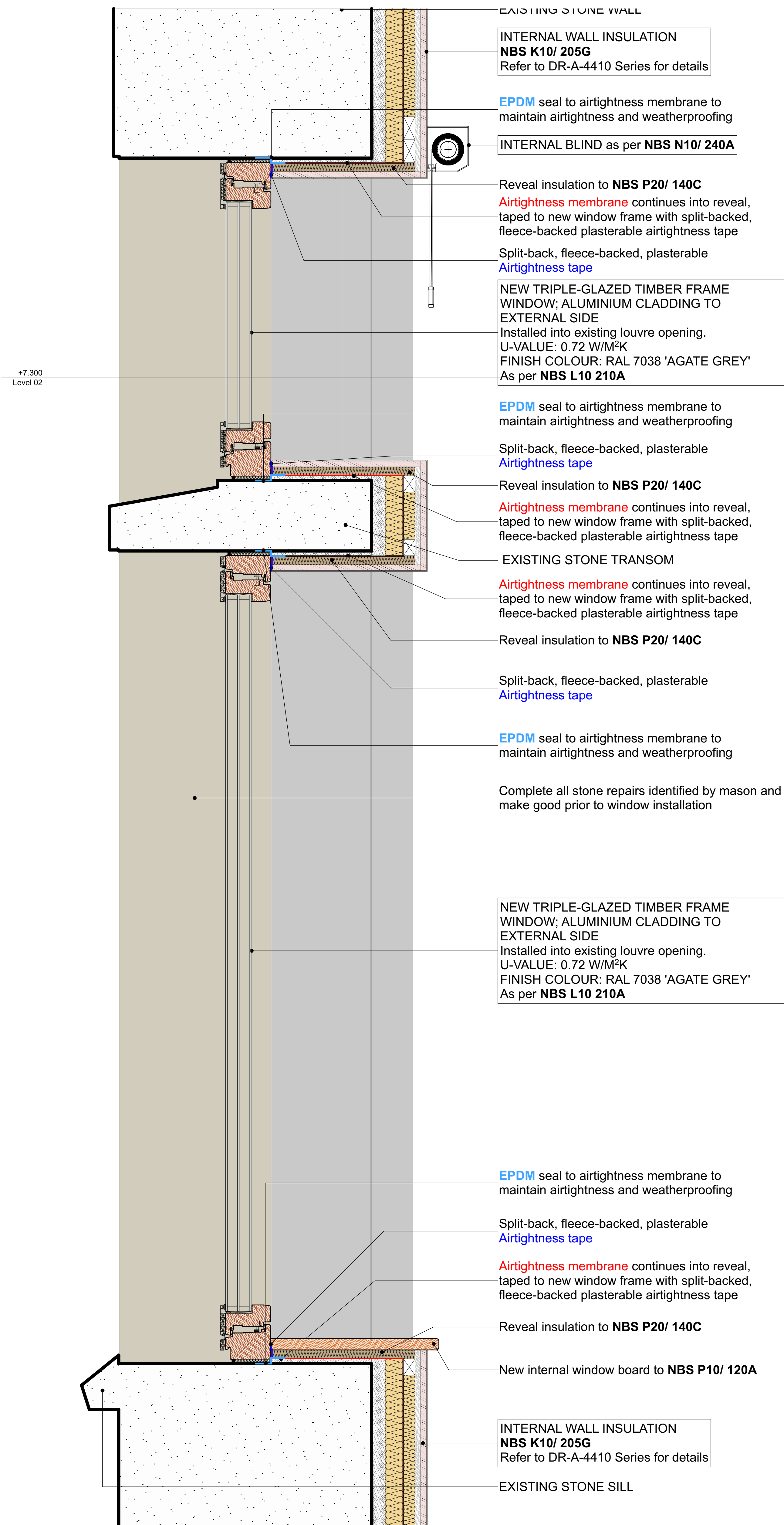
Typical New Side-Hung Outward Opening Window Section Detail 1:5
