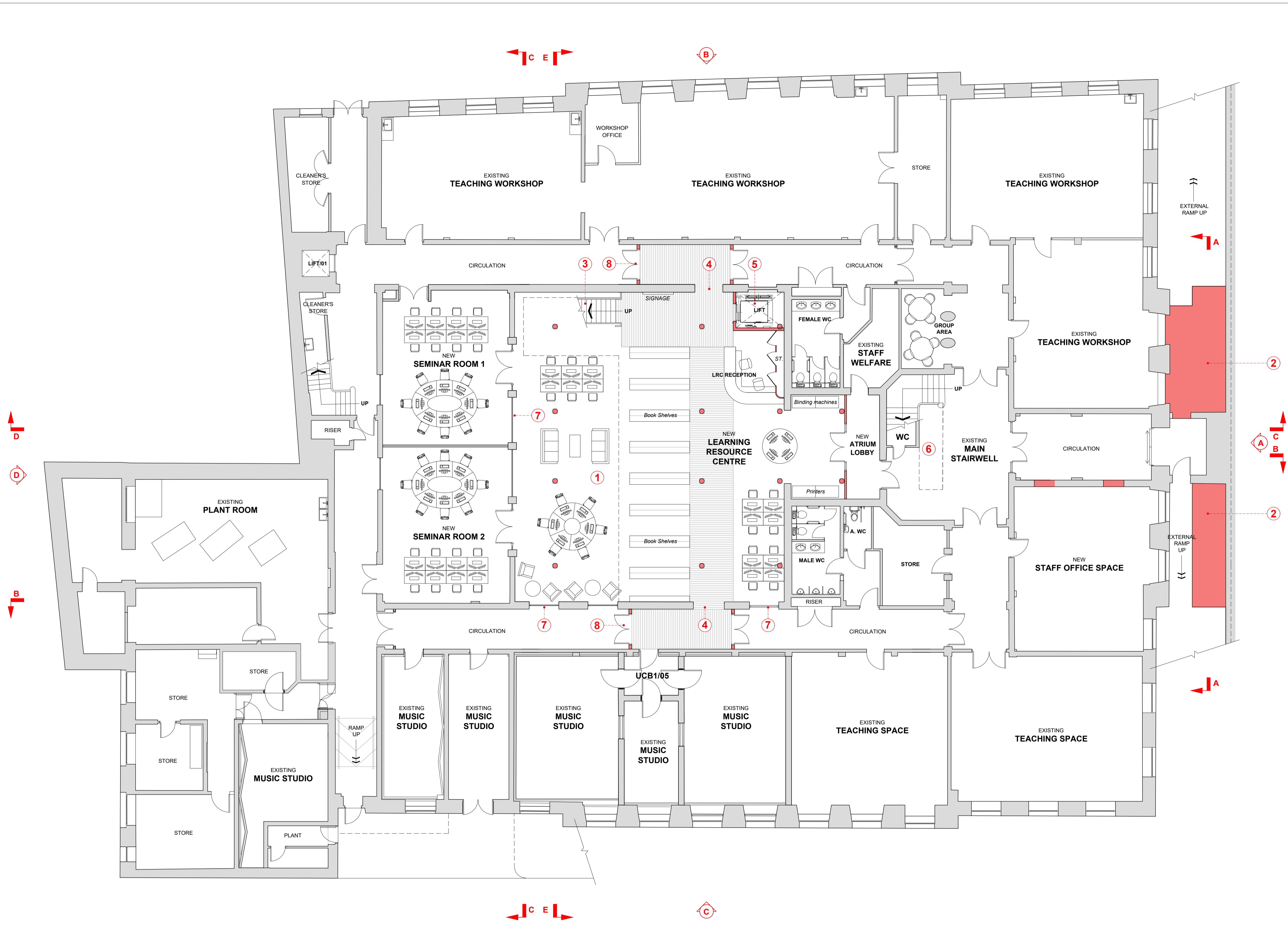
PROPOSED FLOOR PLAN - LEVEL 01 1:100 @ A1
