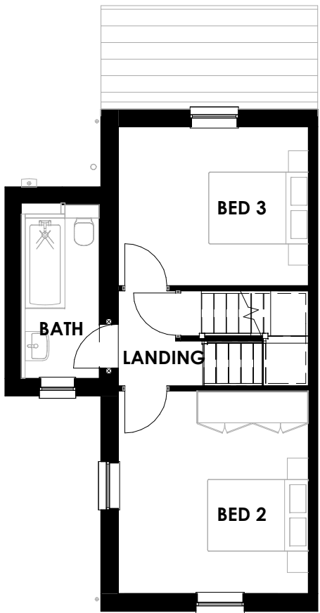
FIRST FLOOR PLANNING 1 : 100
