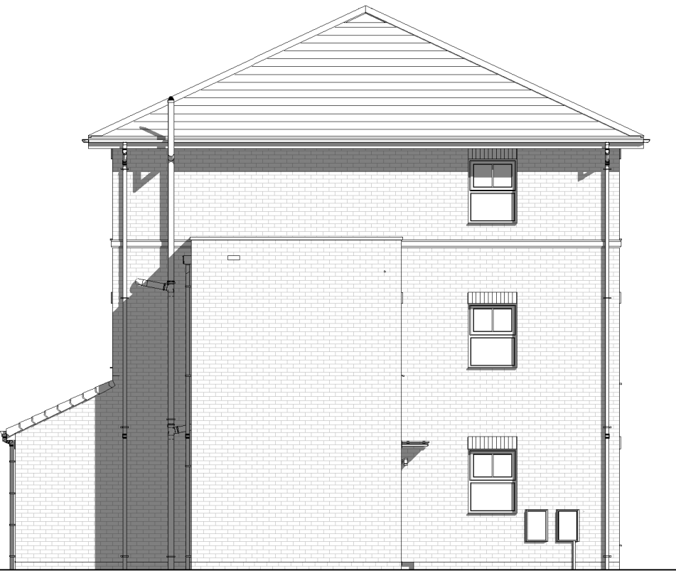
ELEVATION D PLANNING 1 : 100
