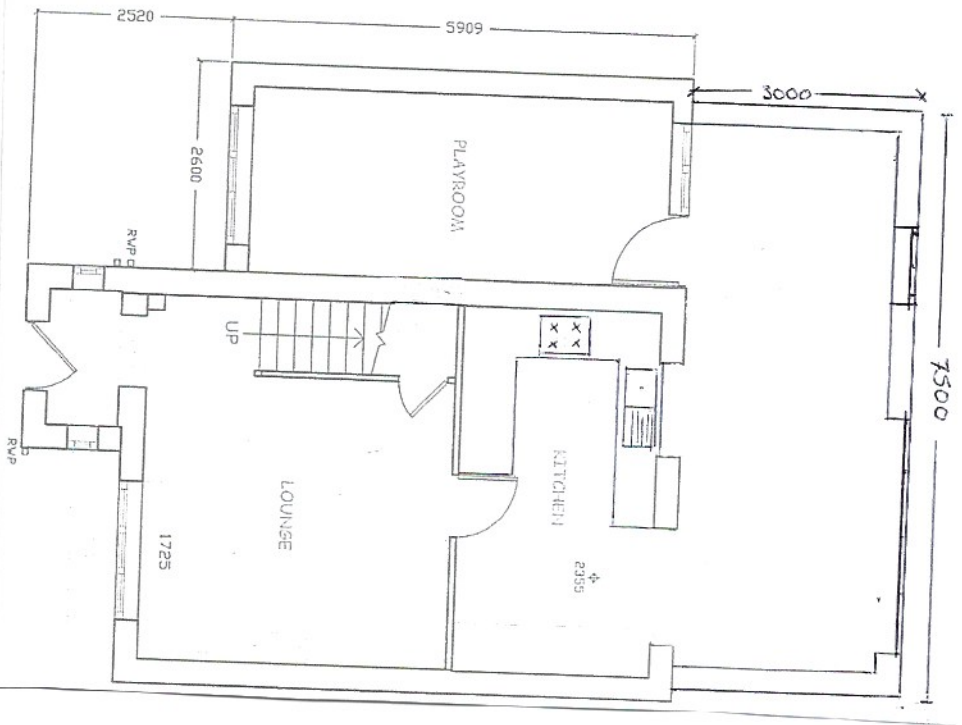
GROUND FLOOR PROPOSED 1:160
