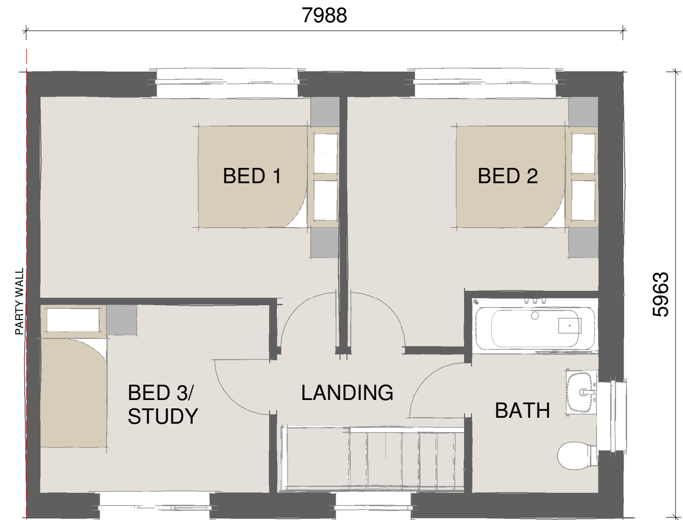
First Floor. 1 : 50
