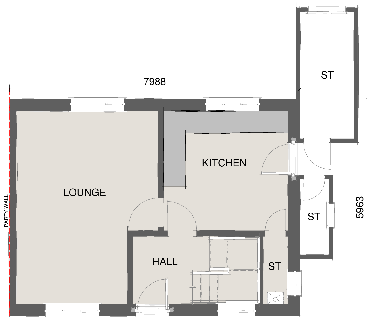
Ground Floor. 1 : 50
