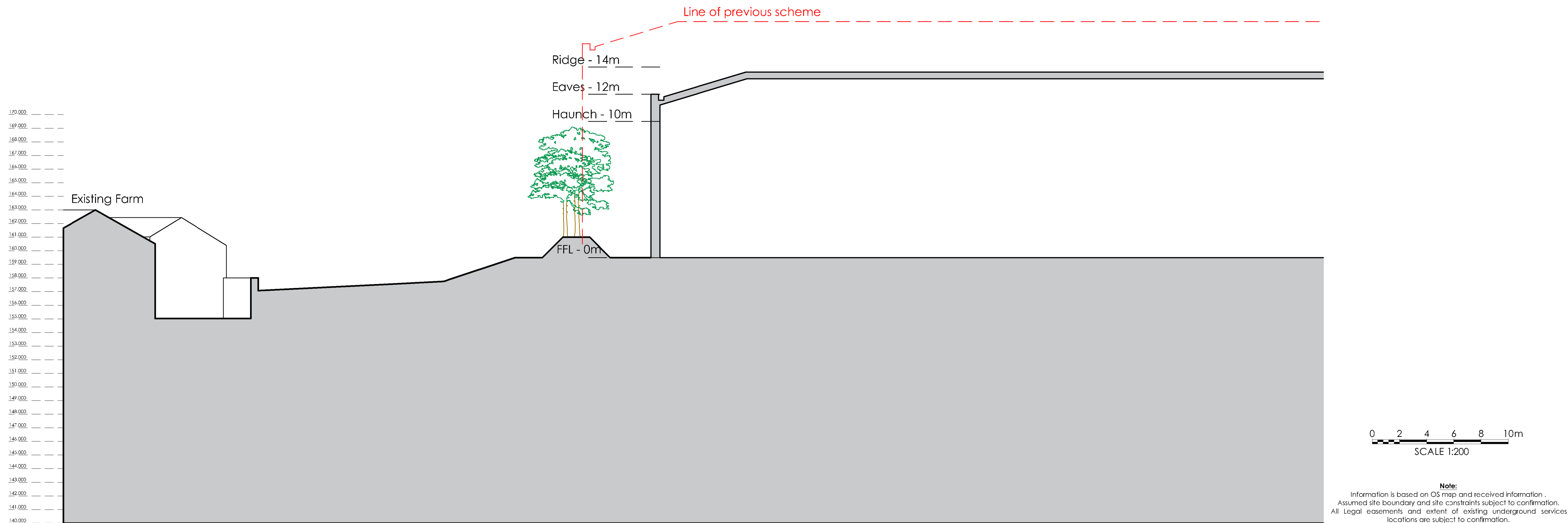
Proposed Site Section B - 45 degrees from existing Lane Side Farmhouse windows (1:200)
