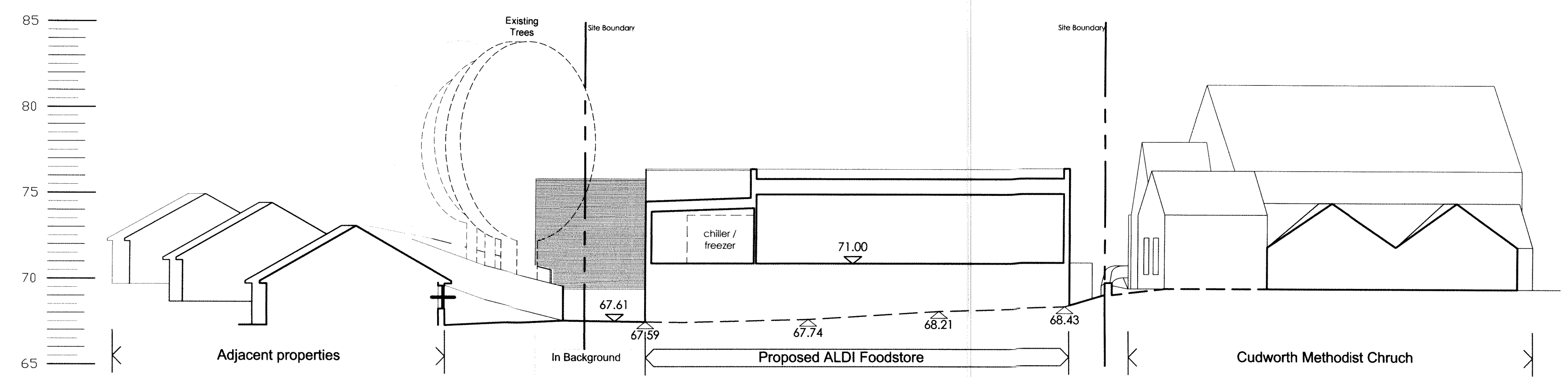
SECTION B - B' - Boundary between warehouse side of foodstore and adjacent dwellings
