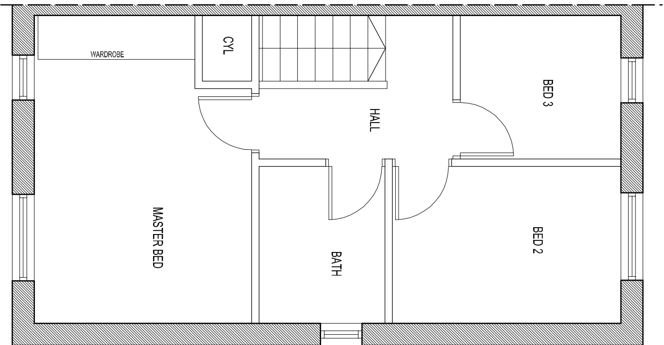
EXISTING FIRST FLOOR PLAN 1:50
