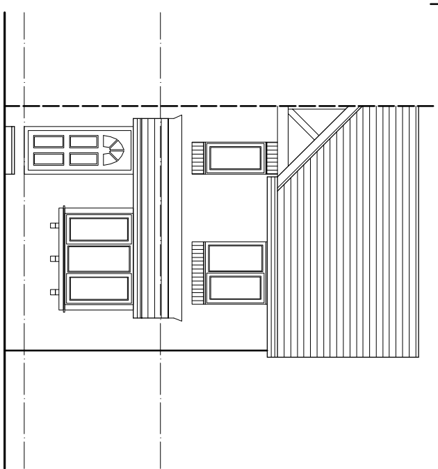
EXISTING EAST ELEVATION 1:100
