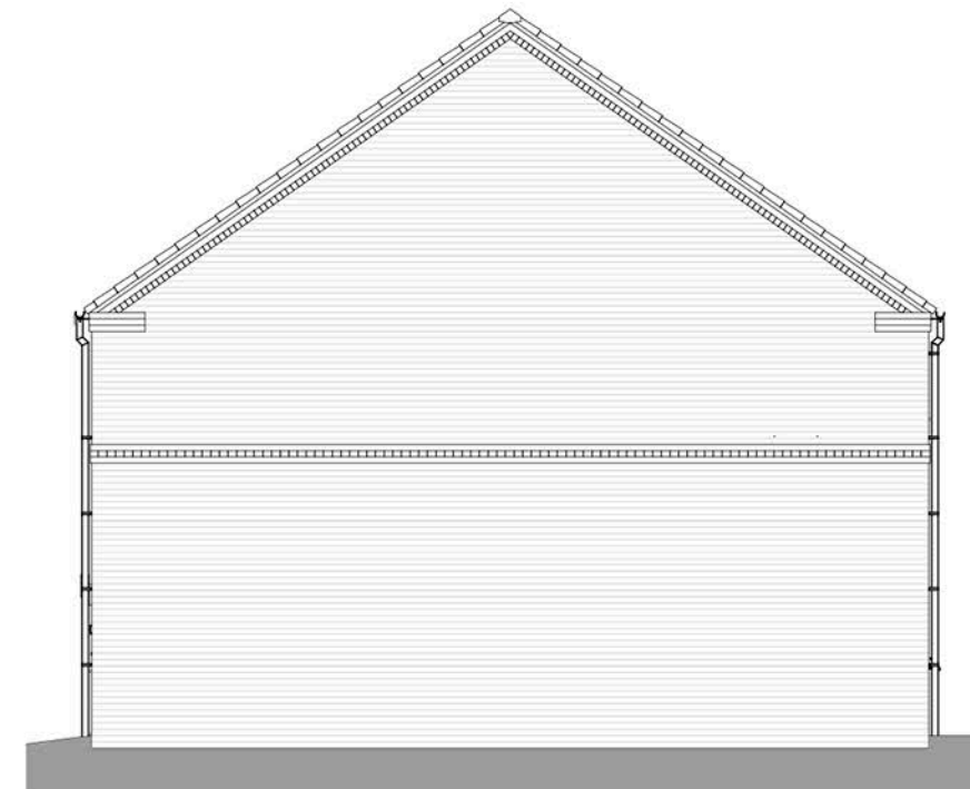
SIDE ELEVATION Kilminster
