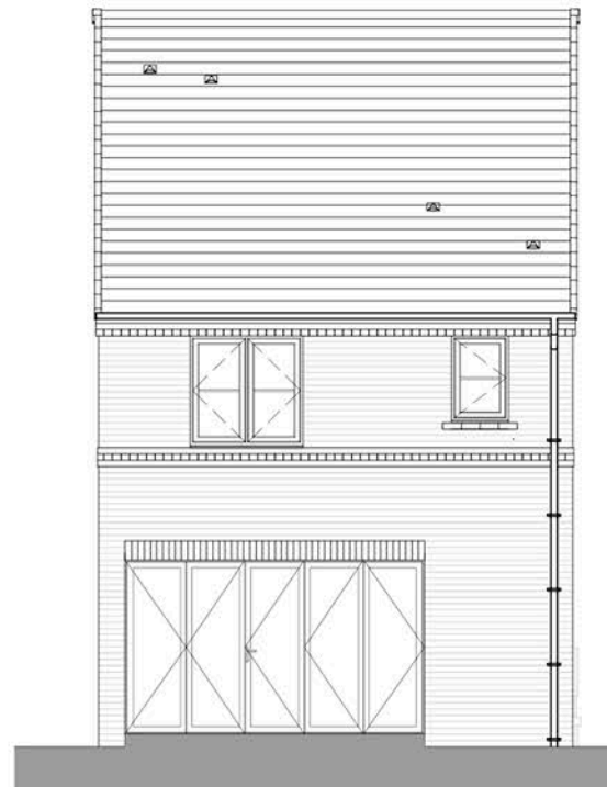
REAR ELEVATION Kilminster
