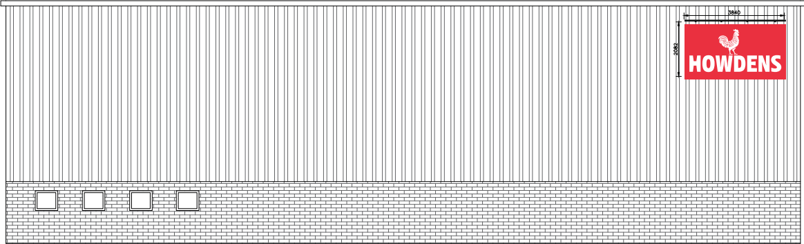
NORTH ELEVATION
