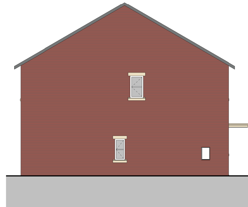
2 Side Elevation 1 : 50
