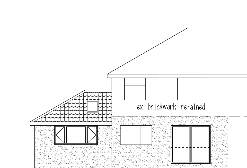
REAR ELEVATION
