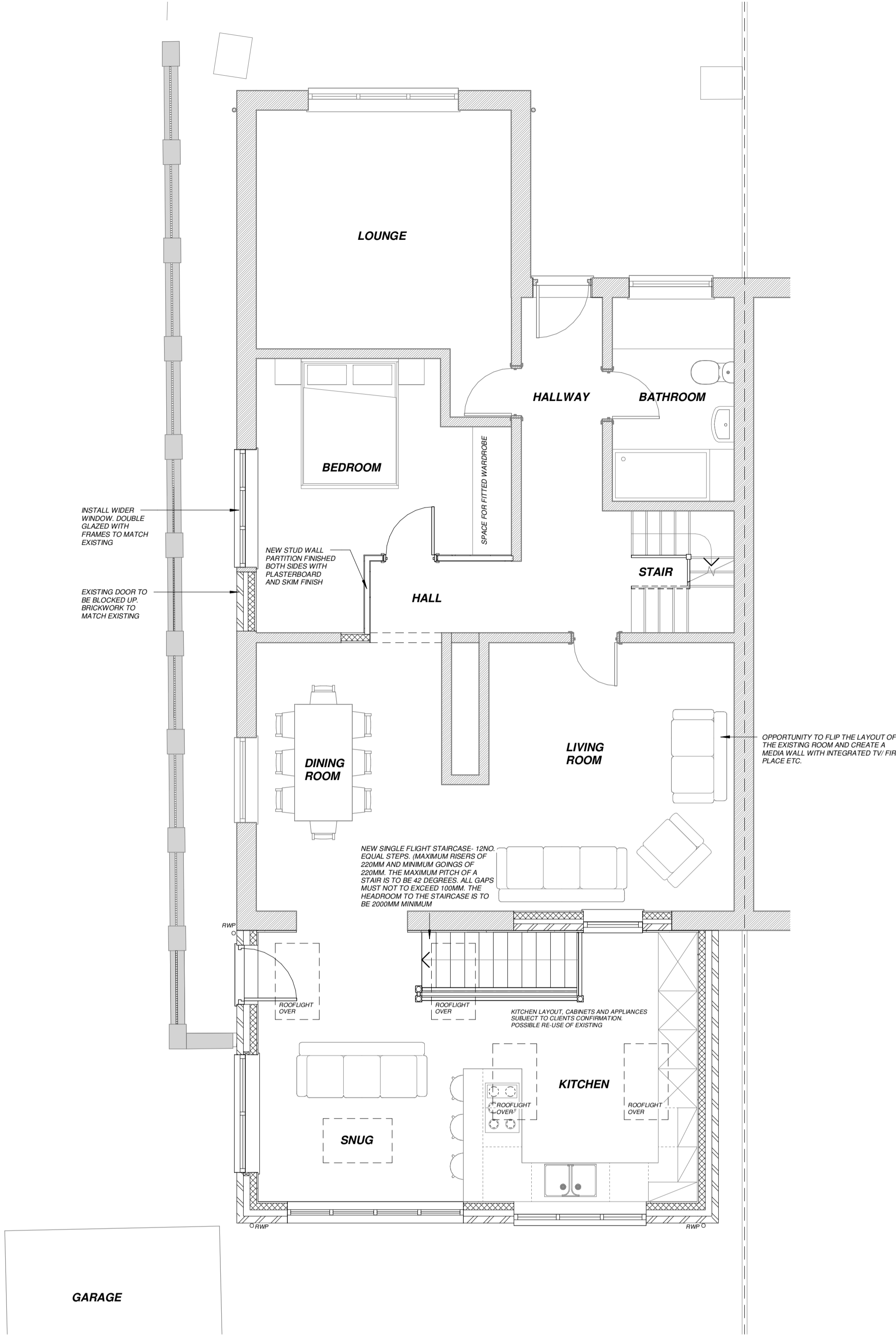
PROPOSED GROUND FLOOR GA PLAN 1 : 50
