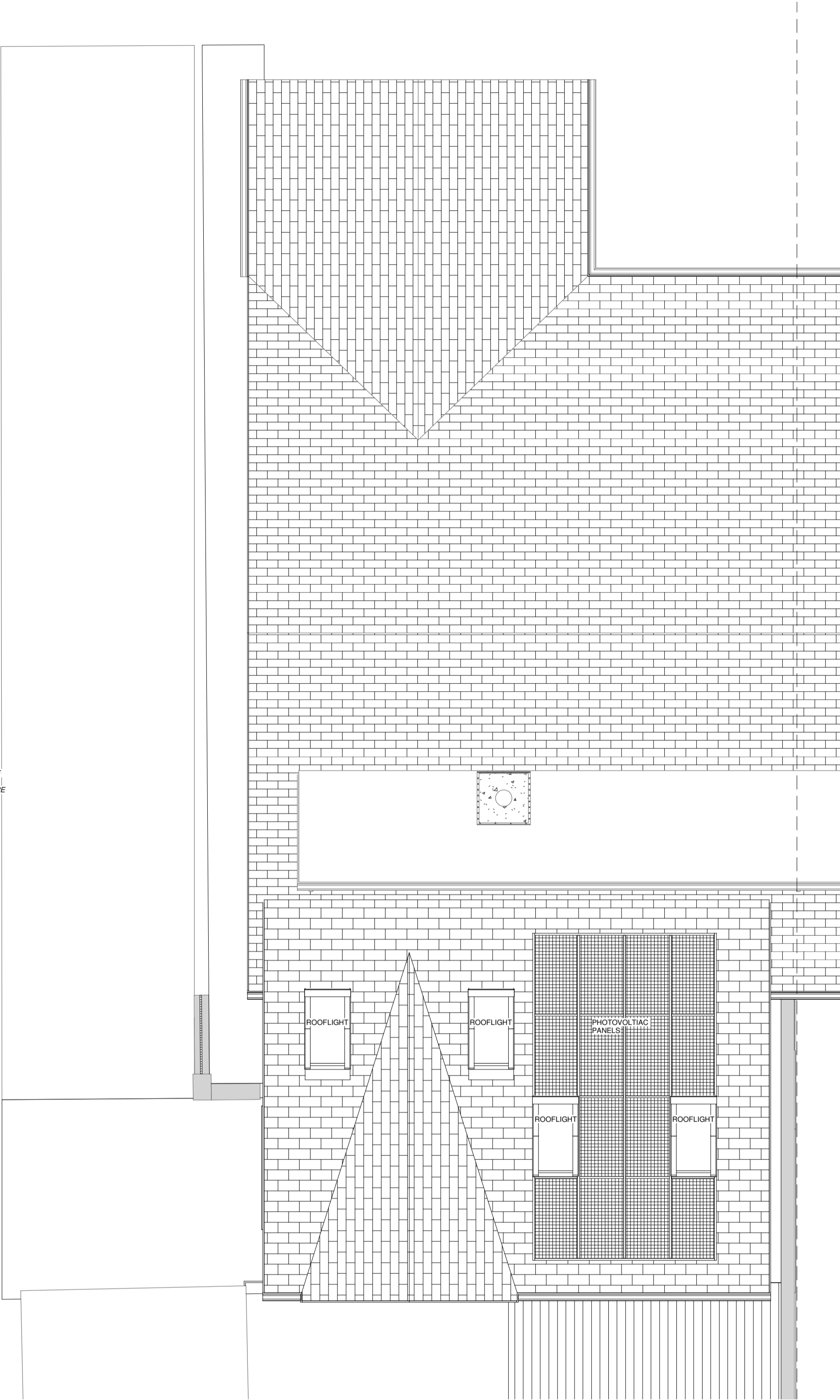
PROPOSED ROOF GA PLAN 1 : 50
