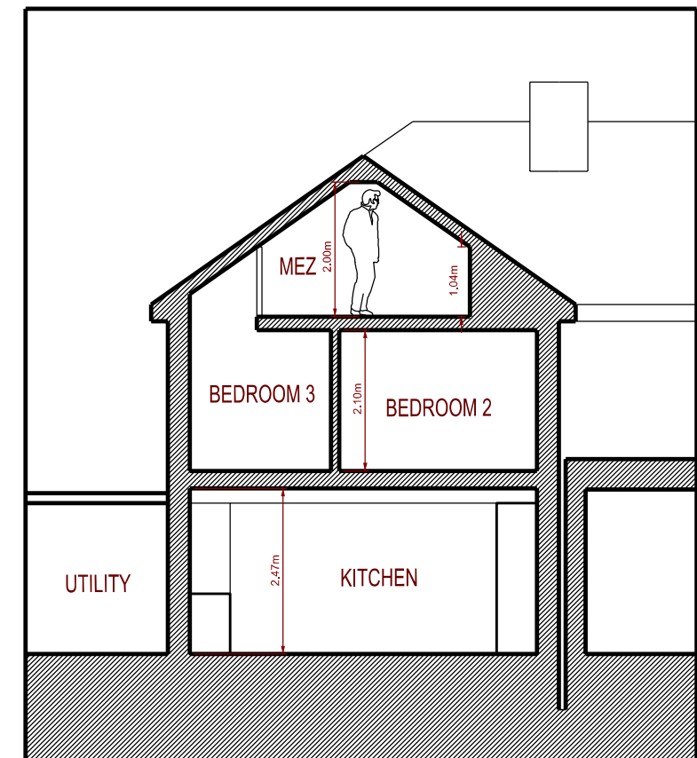
Cross Section
