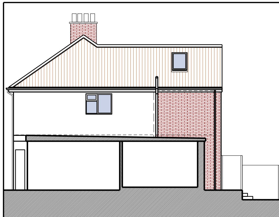
South Elevation
