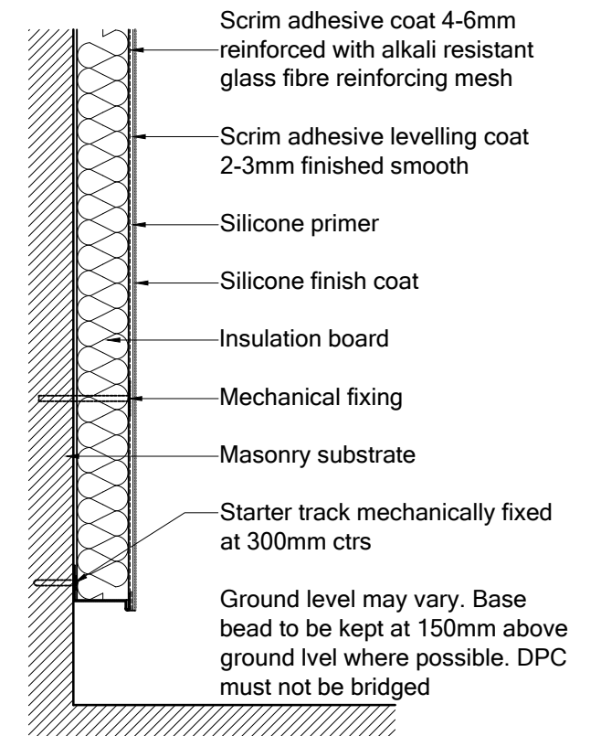
TYPICAL RENDER BASE DETAIL 1:10
