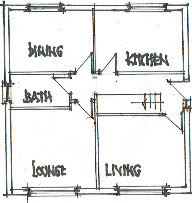
LAYOUT PLANS GROUND FLOOR
