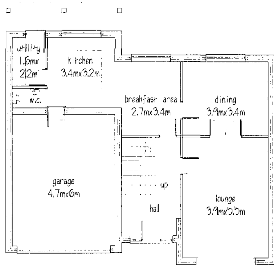
GROUND FLOOR
