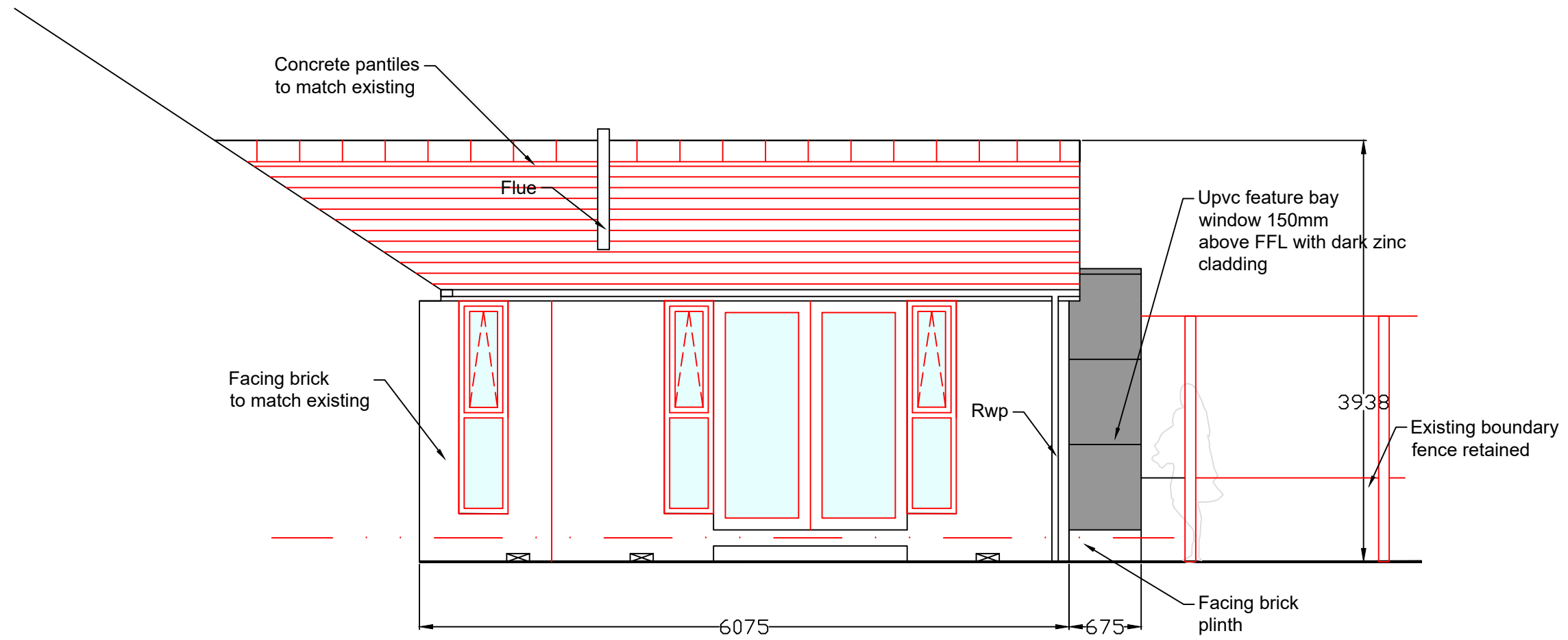
PROPOSED SIDE ELEVATION TO REAR 1:50
